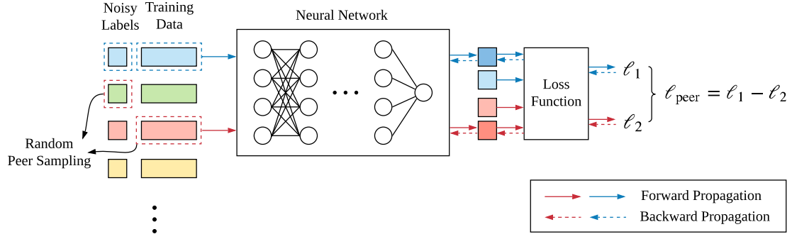
Figure A1. Illustration of our peer loss implementation.
