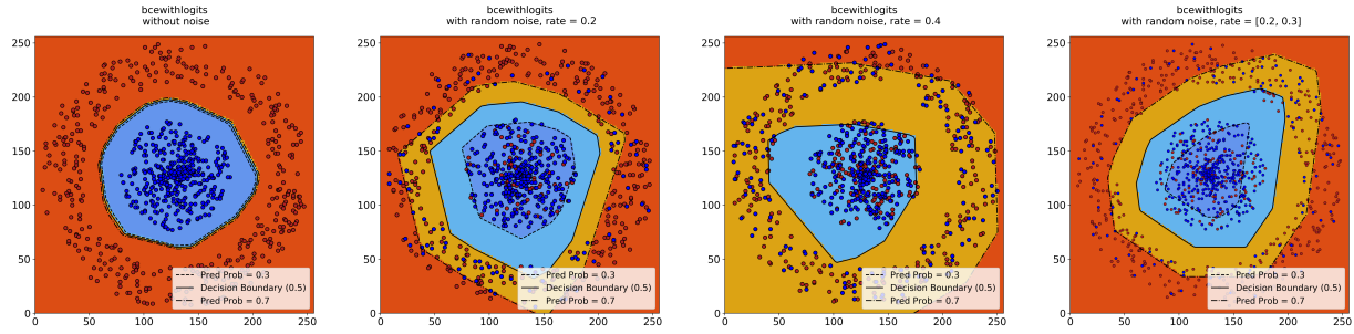
Figure A3. Decision boundary for cross entropy trained on clean and noisy data (Left: trained on noisy labels, e_{+1} = e_{-1} = 0.2 . Middle: trained on noisy labels, e_{+1} = e_{-1} = 0.4 . Right: asymmetric noise e_{+1} = 0.2, e_{-1} = 0.3 ).
