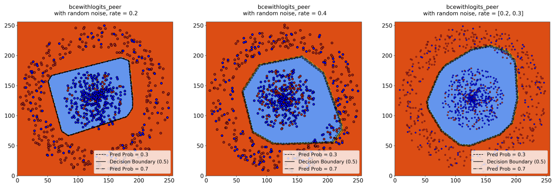
Figure A4. Decision boundary for peer loss. Left: e_{+1} = e_{-1} = 0.2 . Middle: e_{+1} = e_{-1} = 0.4 . Right: asymmetric noise e_{+1} = 0.2, e_{-1} = 0.3
