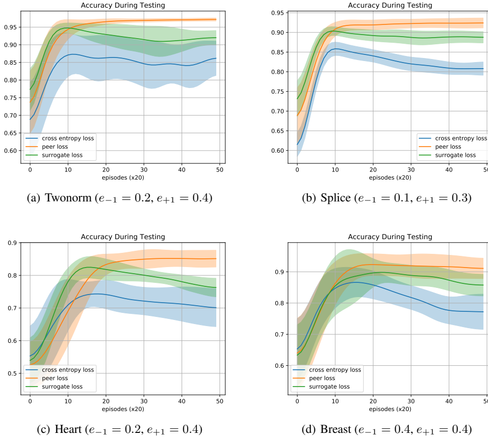
Figure A2. Accuracy on test set during training
