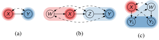
Figure 4. (a, b) Hedges for P_{\mathbf{x}}(\mathbf{y}) where, for both cases, \{\mathbf{Y}\} is the sole root set and the only element of \mathcal{F}' with \mathcal{F} = \mathcal{G} . (c) is not a hedge for P_{\mathbf{x}}(\mathbf{y}) but \{\mathbf{Y}_1, \mathbf{W}\} -rooted c-forests \mathcal{F} = \mathcal{G}\{\{\mathbf{Y}_1, \mathbf{W}, \mathbf{X}\}\} and \mathcal{F}' = \mathcal{G}\{\{\mathbf{Y}_1, \mathbf{W}\}\} form a hedge for P_{\mathbf{x}}(\mathbf{y}) .
