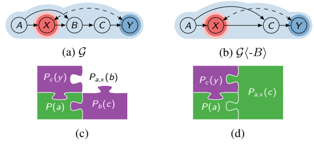
Figure 7. Causal graphs (a) \mathcal{G} and (b) \mathcal{G}(-B) . Corresponding gc-factors (c, d) represented as puzzle where identified factors are colored with green, P_X(A, C) , and purple, P(B, C, Y) . 4
