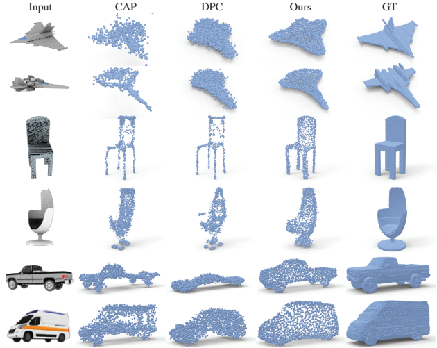
Figure 8. Qualitative comparison with differentiable renderers for point clouds.
