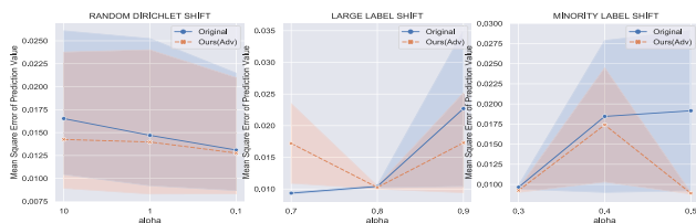
Figure 7. The prediction mean square error of 1D sprite position prediction (lower is better). (a) Random Dirichlet shift, where the smaller \alpha corresponding to the bigger shift. (b) Large target shift, where \alpha is the possibility of shifted label. (c) Minority shift, where \alpha is the ratio of minority classes.
