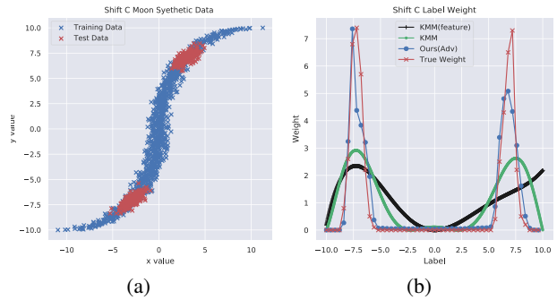
Figure 5. (a) The illustration of Moon Synthetic Data (Shift C), where the generated two quarter circles training set as blue symbols show. (b) The visualization of label weight P_Y^T / P_Y^S of KMM, KMM(feature), our framework and the Ground Truth.
