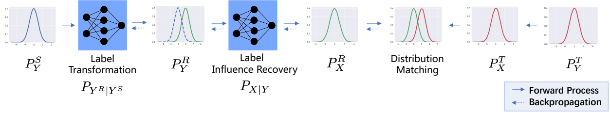
Figure 1. The illustration of the LTF framework. Here we make an example which assumes that X = Y + \epsilon . Firstly, the Label Transformation Model LT transforms the training label distribution P_Y^S (blue one) to a new label distribution P_Y^R (green one), and then the Label Influence Recovery Model G generates the sample distribution P_X^R from the data generated from P_Y^R . By matching the target sample distribution P_X^T (red one) and P_X^R and fixing the G , the P_Y^R from LT is expected to be close to P_Y^T . As such, the target label distribution P_Y^T can be approximated by P_Y^R .
