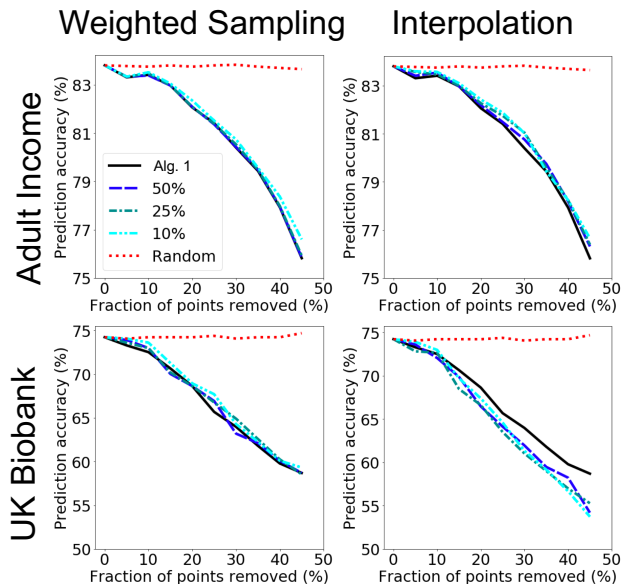
Figure 1. Point removal performance. Given a data set and task, we iteratively remove a point, retrain the model, and evaluate its performance. Each curve corresponds to a different point removal order, based on the estimated distributional Shapley values (compared to random). For example, the 10% curve corresponds to estimating values with 10% of the baseline computation of Algorithm 1. We plot classification accuracy vs. fraction of data points removed from the training set, for each task and each optimization method.
