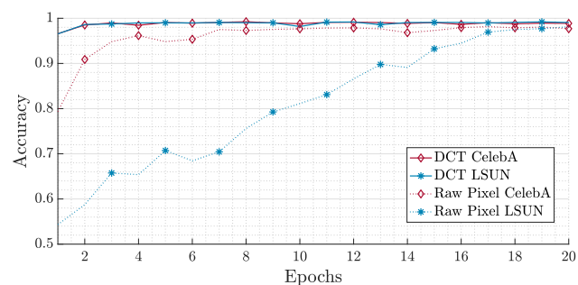
Figure 6: Validation accuracy for our CNN-classifier. We report the validation accuracy during training for the first 20 epochs.
