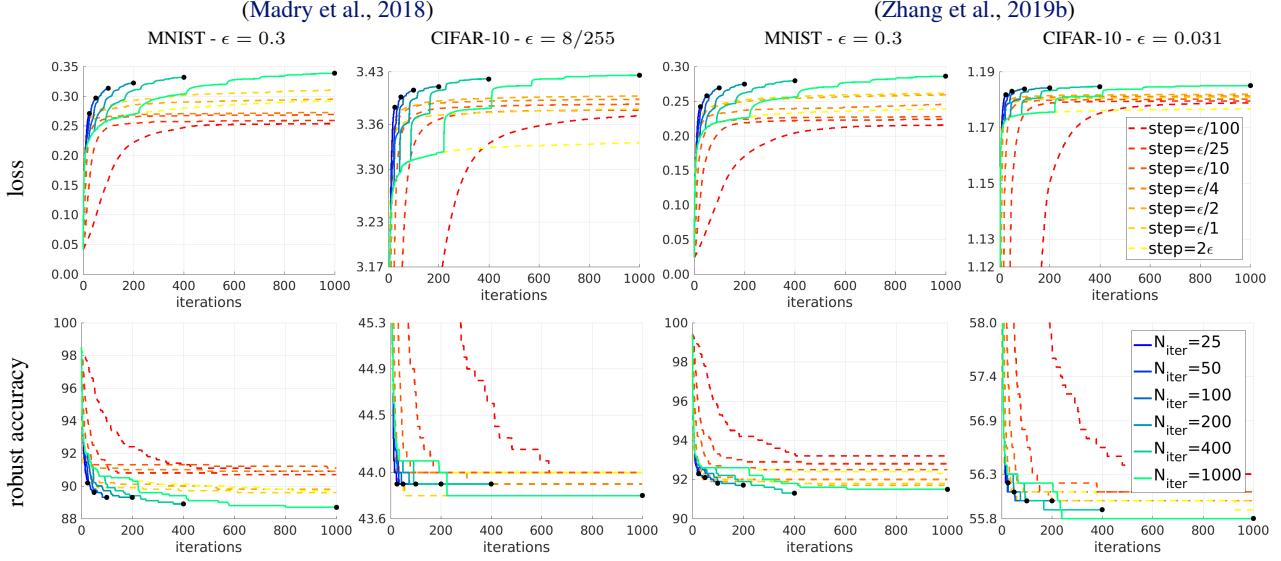
Figure 1. PGD with Momentum vs APGD : best cross-entropy loss (top) and robust accuracy (bottom) obtained so far as function of iterations for the models of (Madry et al., 2018) and TRADES (Zhang et al., 2019b) for PGD with a momentum term ( \mu = 0.75 , as used in APGD) (dashed lines) with different fixed step sizes (always 1000 iterations) and APGD (solid lines) with different budgets of iterations. APGD outperforms PGD with Momentum for every budget of iterations in achieved loss and almost always in robust accuracy.
