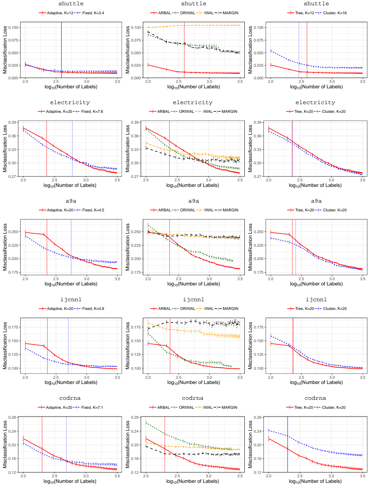
Figure 7: Misclassification loss on hold out test data versus number of labels requested (log 10 scale). Left: ARBAL with fixed and adaptive threshold \gamma . Middle: ARBAL, RIWAL, IWAL, and MARGIN. Right: ARBAL with different partitioning methods: binary tree and hierarchical clustering. For \kappa = 20 and \tau = 800 , dataset shuttle, electricity, a9a, ijcnn1, codrna. For left and right plots, we give the average number of resulting regions K in the legend. The vertical lines indicate when ARBAL transits from the first to the second phase.
