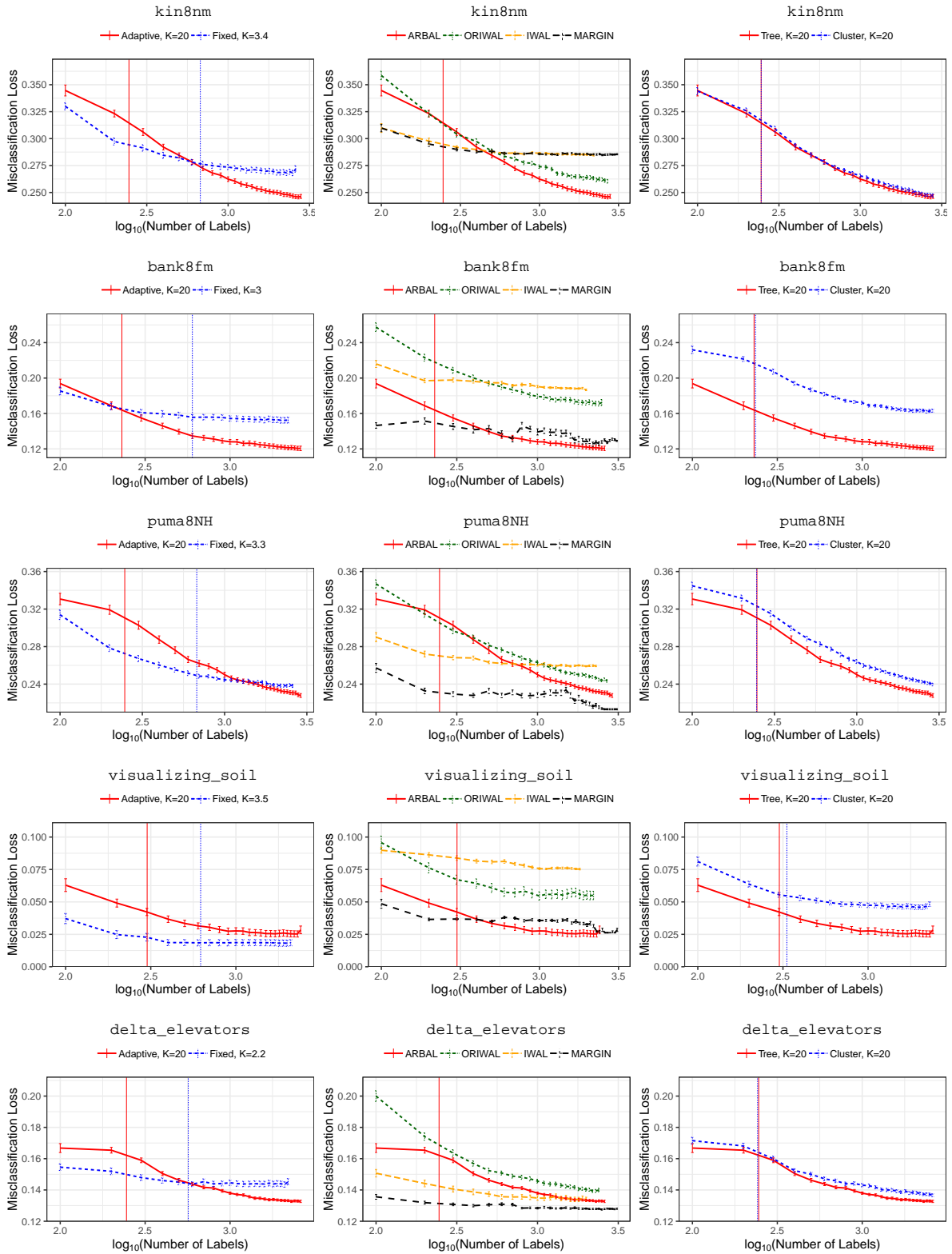
Figure 4: Misclassification loss on hold out test data versus number of labels requested ( \log_{10} scale). Left: ARBAL with fixed and adaptive threshold \gamma . Middle: ARBAL, RIWAL, IWAL, and MARGIN. Right: ARBAL with different partitioning methods: binary tree and hierarchical clustering. For \kappa = 20 and \tau = 800 , dataset kin8nm, bank8fm, puma8NH, visualizing soil, delta elevators. For left and right plots, we give the average number of resulting regions K in the legend. The vertical lines indicate when ARBAL transits from the first to the second phase.
