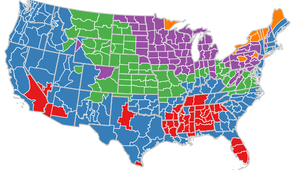
Figure 2. Learnability recovered for the 344 climate divisions. n_i observations. Response Y_i from the i th data domain is
