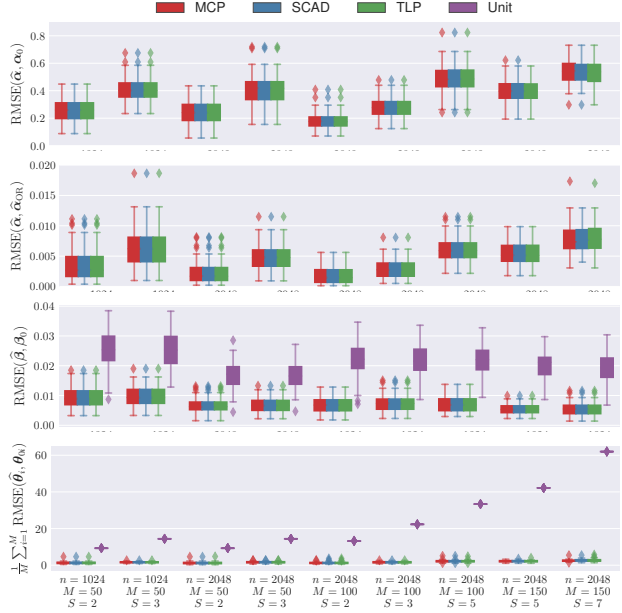
Figure 5. Evaluation of parameter estimation.
