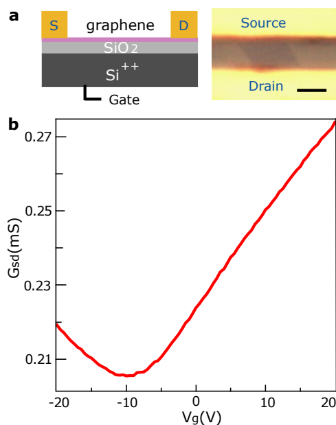
Figure 2. (a) The scheme of the graphene-based FET device (left) and a typical optical image of the device (right, the scale bar is 2 microns). (b) The G_{\text{sd}}-V_g curve of the N-doped graphene device.
