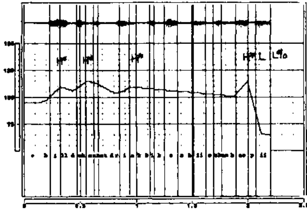
Figure 1. Declarative Contour
