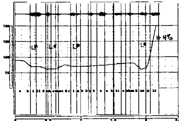
Figure 2. Interrogative Contour
