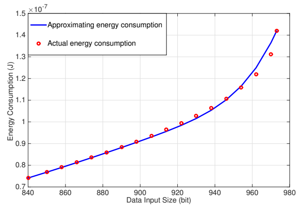
Figure 4: Approximation \hat{G}_{loc} with P_b = 1 W and T = 0.035 s.
