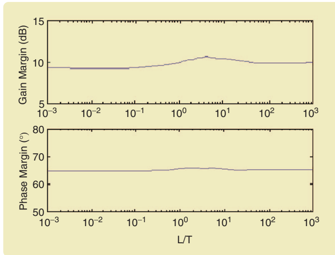
FIGURE 5 Gain and phase margins resulting from PIDEasy designs for first-order delayed plants with various L/T ratios. While requirements of fast transient response, no overshoot, and zero steady-state error are accommodated by time-domain criteria, multiobjective design goals provide frequency-domain margins in the range of 9–11 dB and 65–66°.
