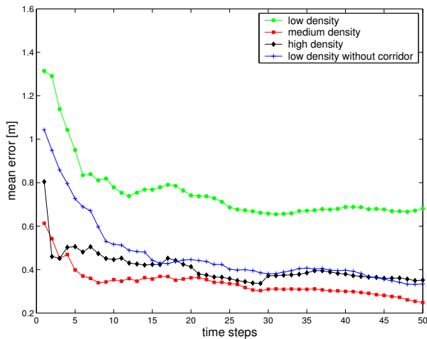
Fig. 6. Impact of the density of RFID transponders on the localization accuracy when our snapshot-based method is used. For the lowest density, results are additionally plotted after removing trials that were performed under adverse conditions (narrow corridor with very few transponders visible).
