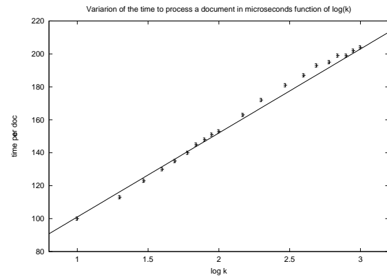
Figure 6: Influence of the k parameter
