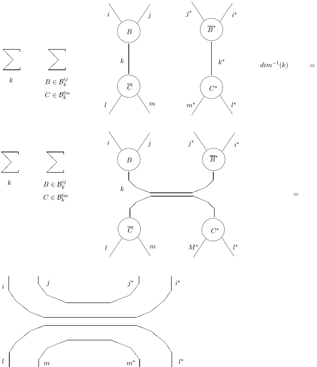
Figure 24: Joining blobs which share one tetrahedron
