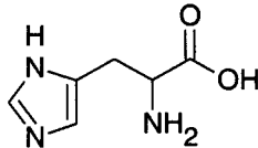
Histidine (His)
