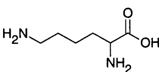
Lysine (Lys)
