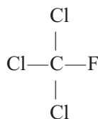
Trichlorofluoromethane
