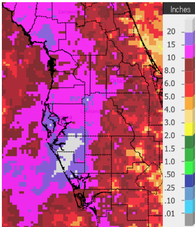
August 1-27, 2024 Rainfall
