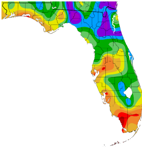
Temperature (F) 8/1/2024 - 8/27/2024
