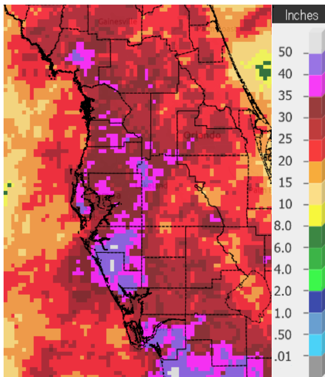
Total Rainfall
