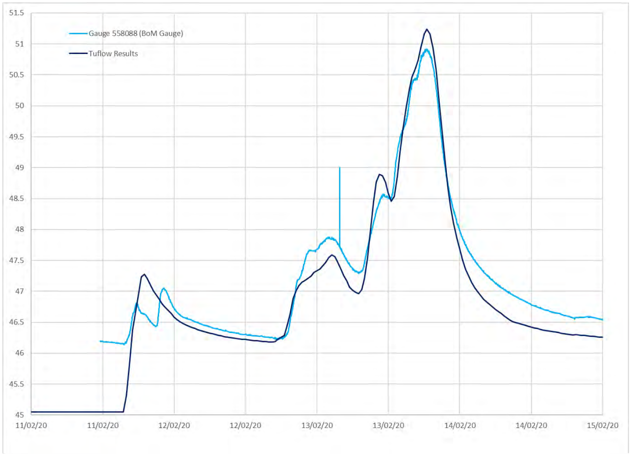
Diagram 112: 2020 Comparison of Water Level at Tyalum Bridge
