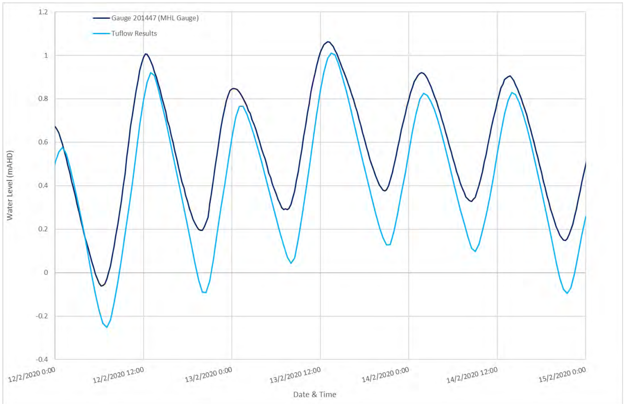
Diagram 110: 2020 Comparison of Water Level at Terranora Gauge
