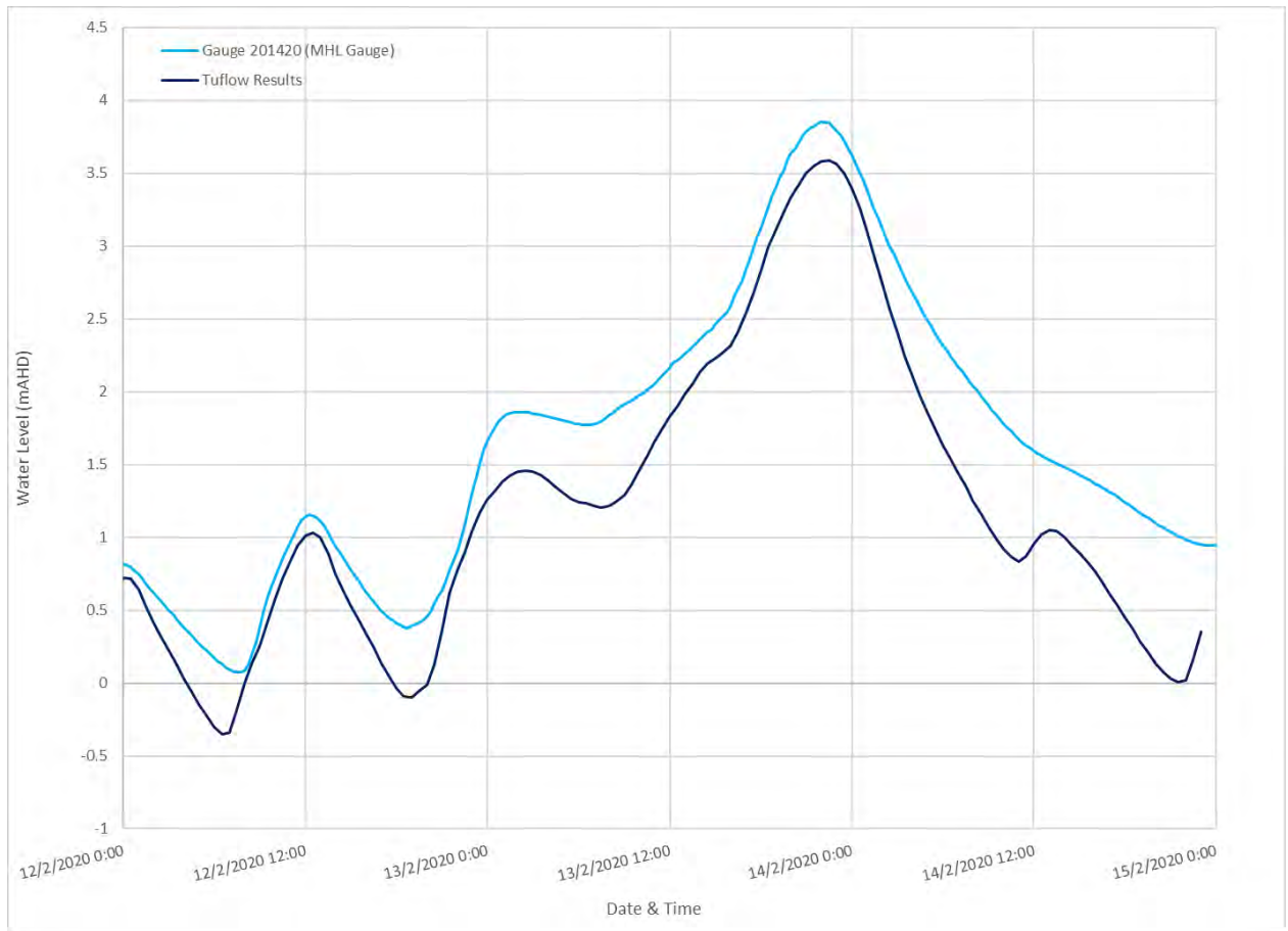
Diagram 107: 2020 Comparison of Water Level at North Murwillumbah
