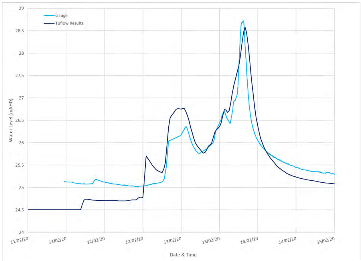
Diagram 113: 2020 Comparison of Water Level at Chillingham Bridge
