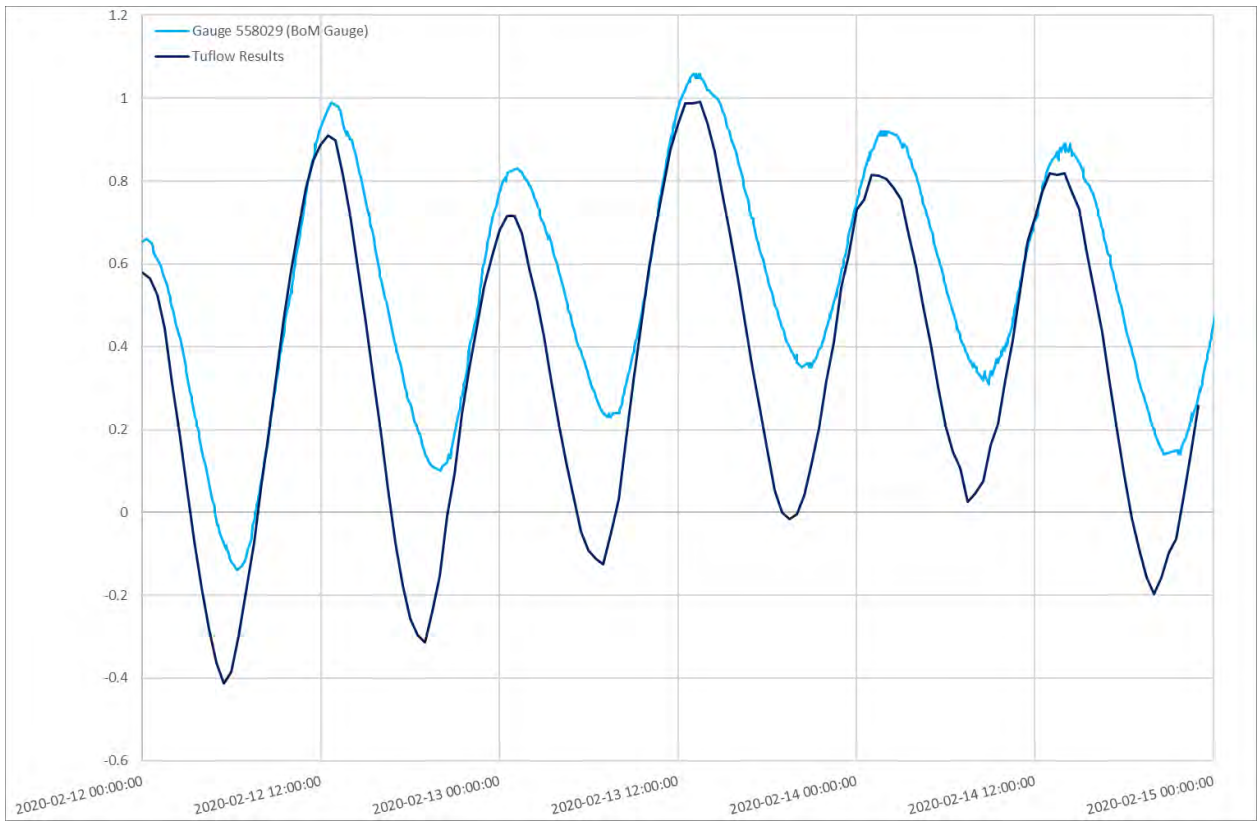
Diagram 111: 2020 Comparison of Water Level at Dry Dock Gauge
