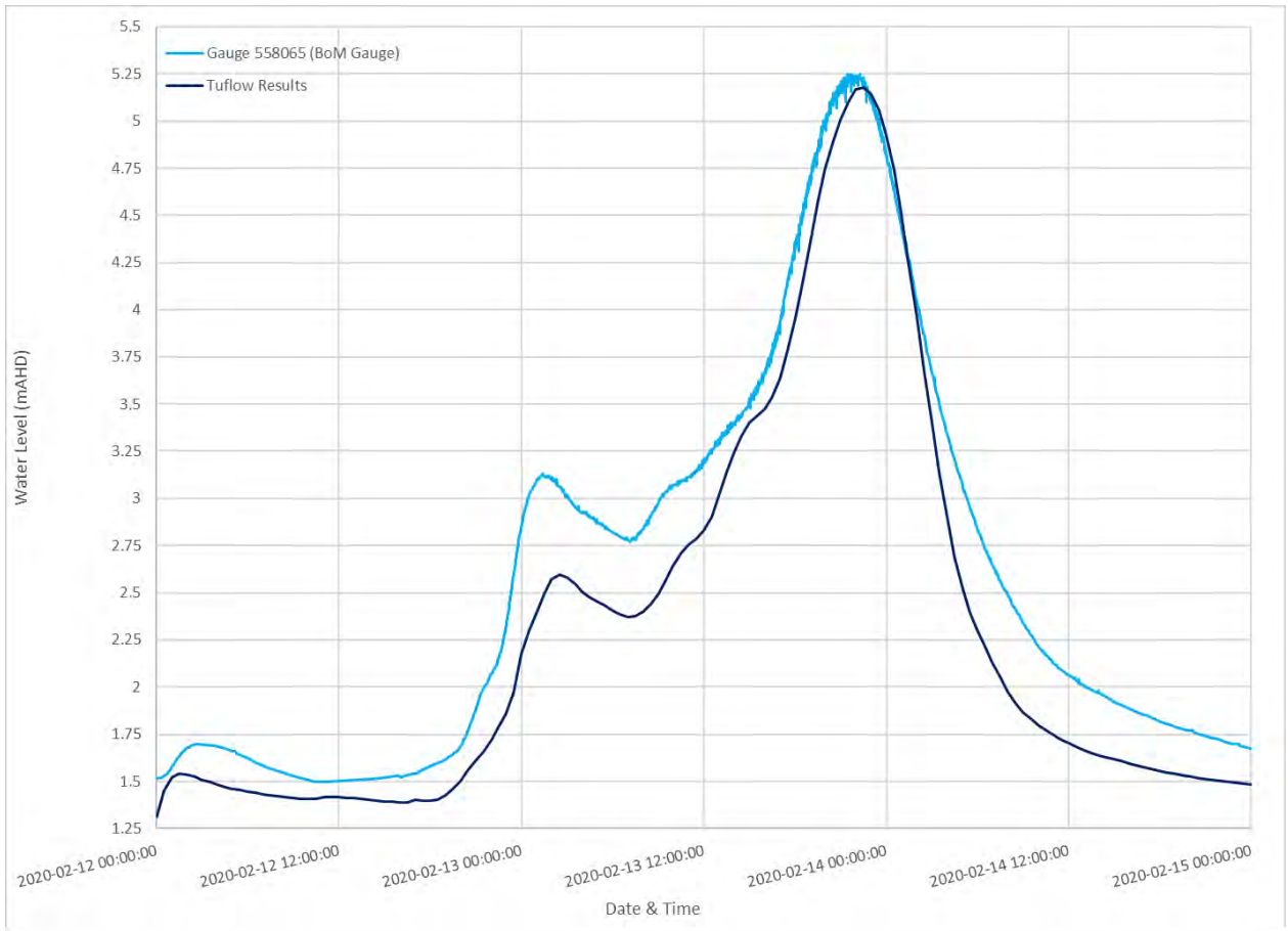
Diagram 105: 2020 Comparison of Water Level at Bray Park Weir Gauge
