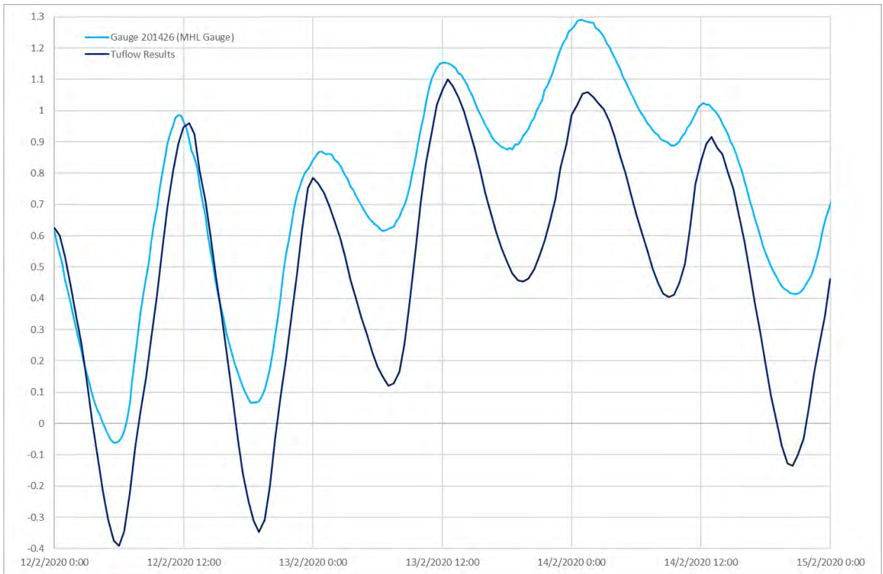
Diagram 109: 2020 Comparison of Water Level at Barney's Point Gauge
