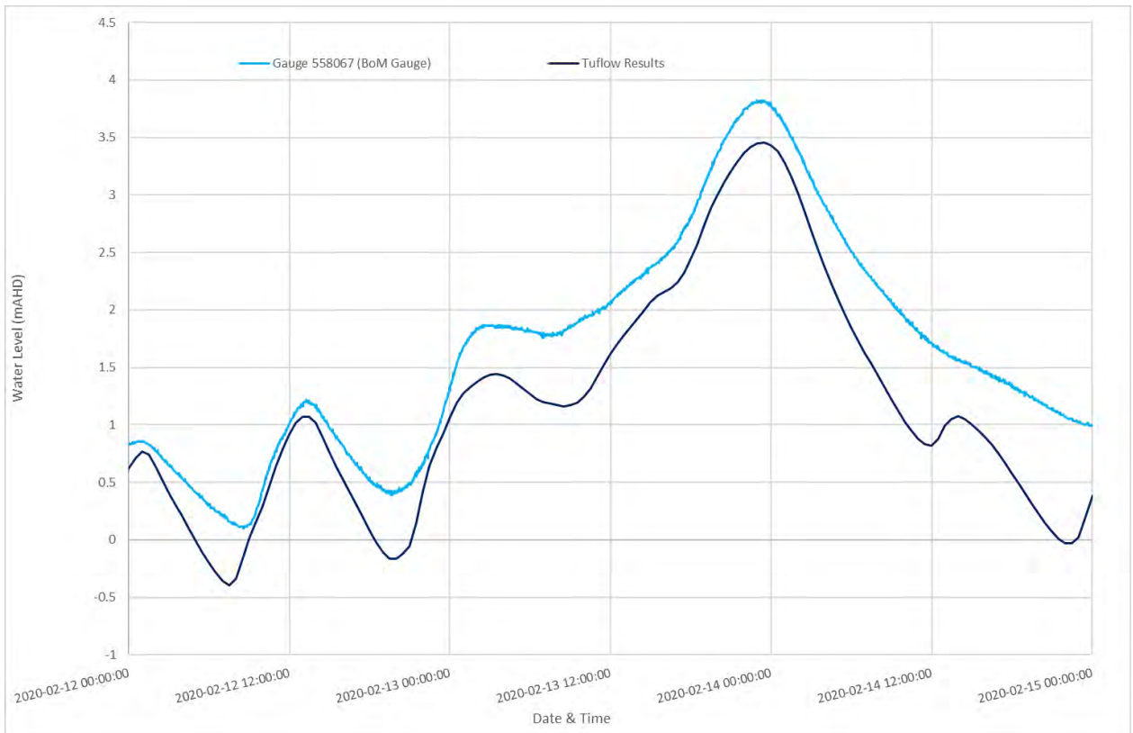
Diagram 106: 2020 Comparison of Water Level at Murwillumbah Bridge
