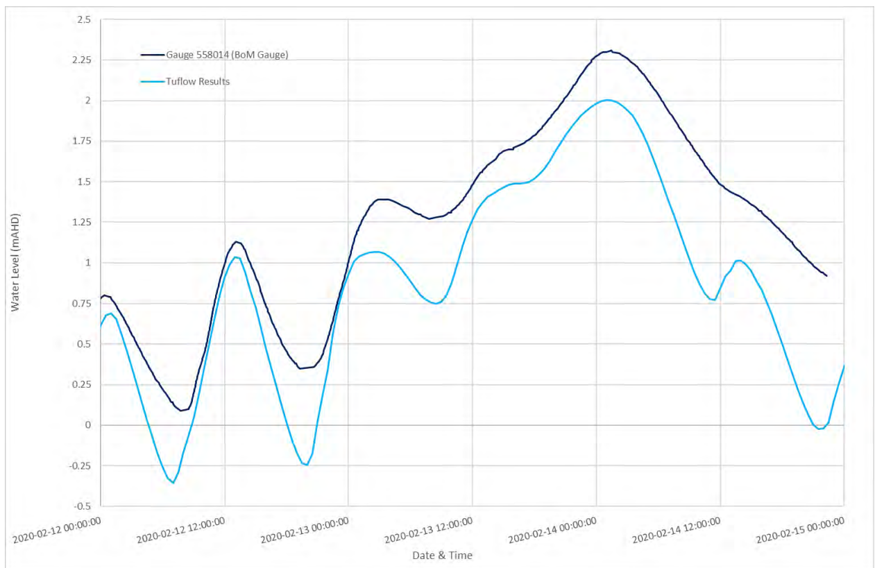
Diagram 108: 2020 Comparison of Water Level at Tumbulgum Gauge
