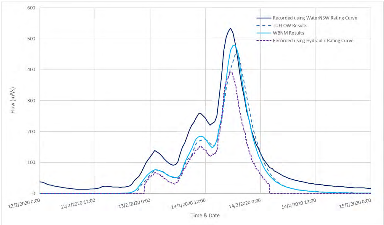
Diagram 95: 2020 Comparison of Flow at Palmers Road
