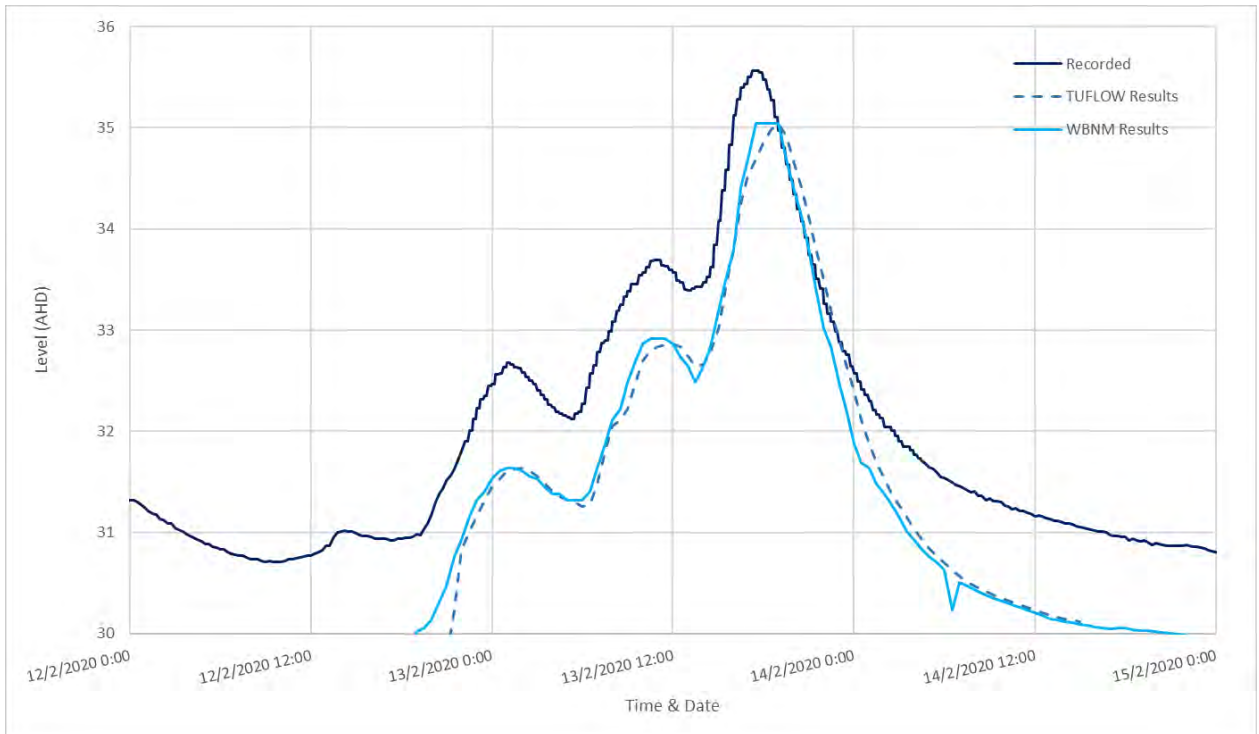
Diagram 100: 2020 Comparison of Water Level at Palmers Road
