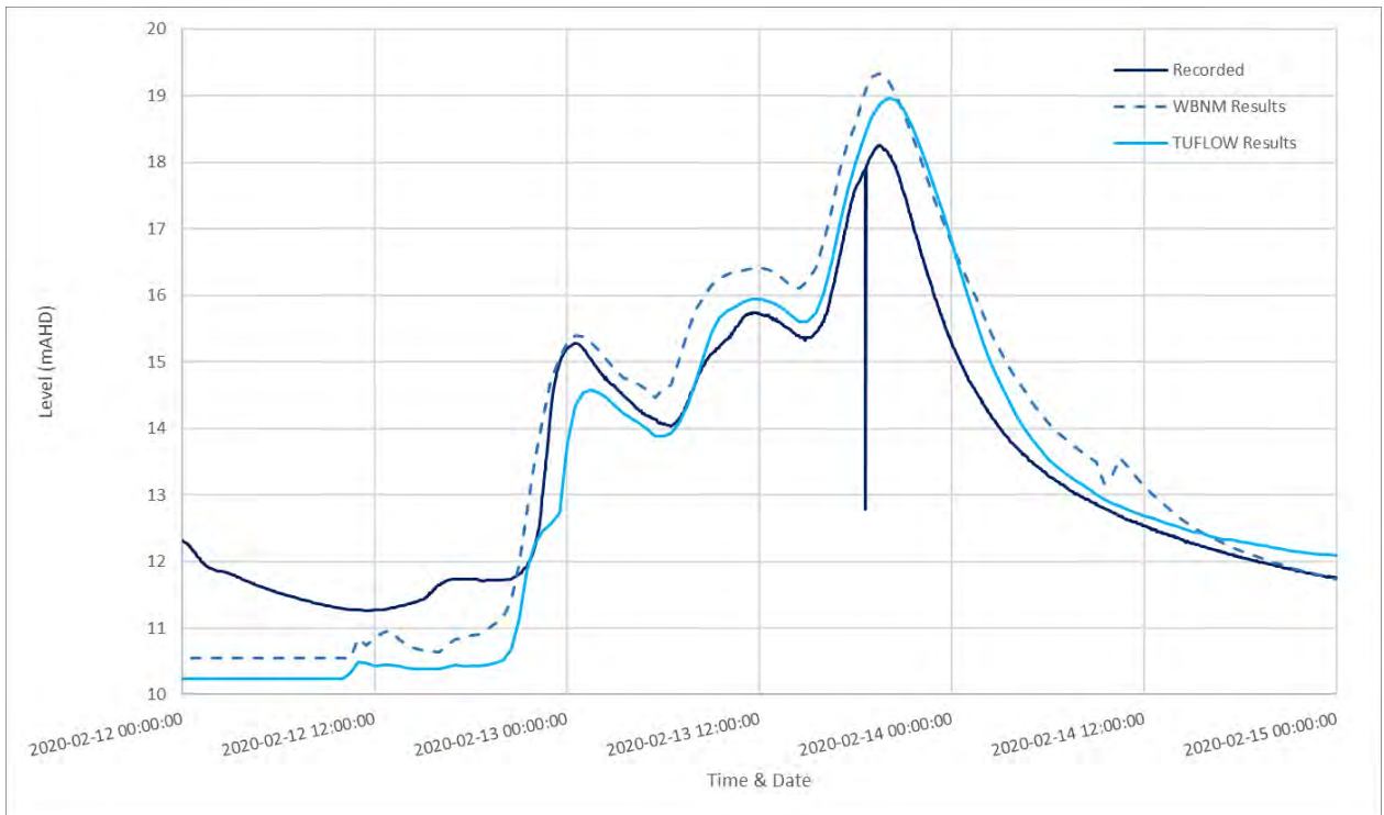
Diagram 101: 2020 Comparison of Water Level at Uki
