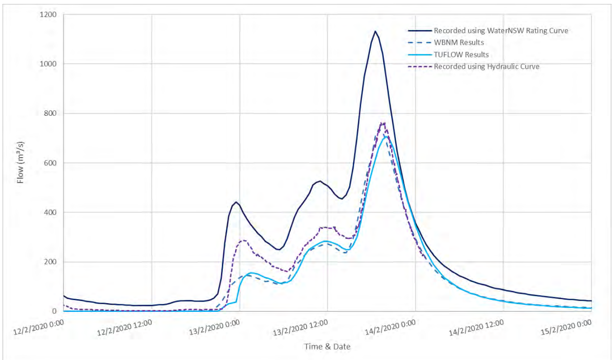
Diagram 96: 2020 Comparison of Flow at Uki
