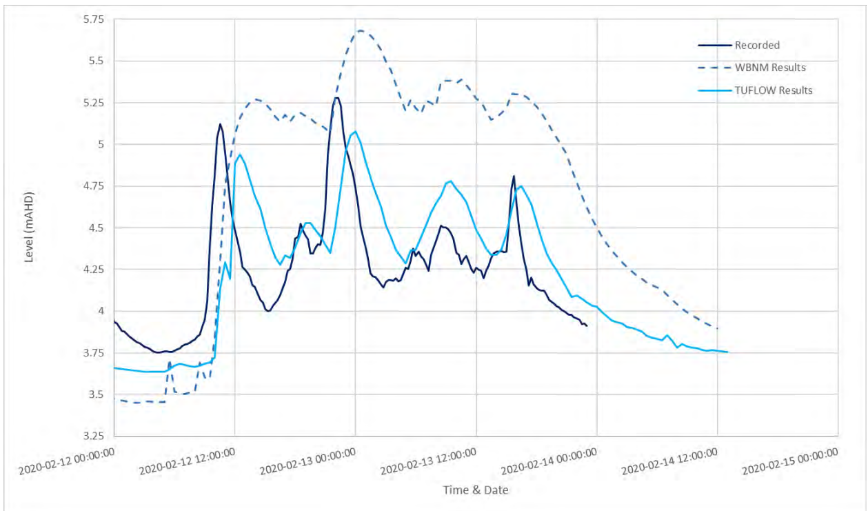
Diagram 104: 2020 Comparison of Water Level at Cobaki Creek
