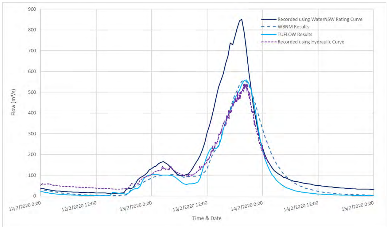
Diagram 97: 2020 Comparison of Flow at Eungella
