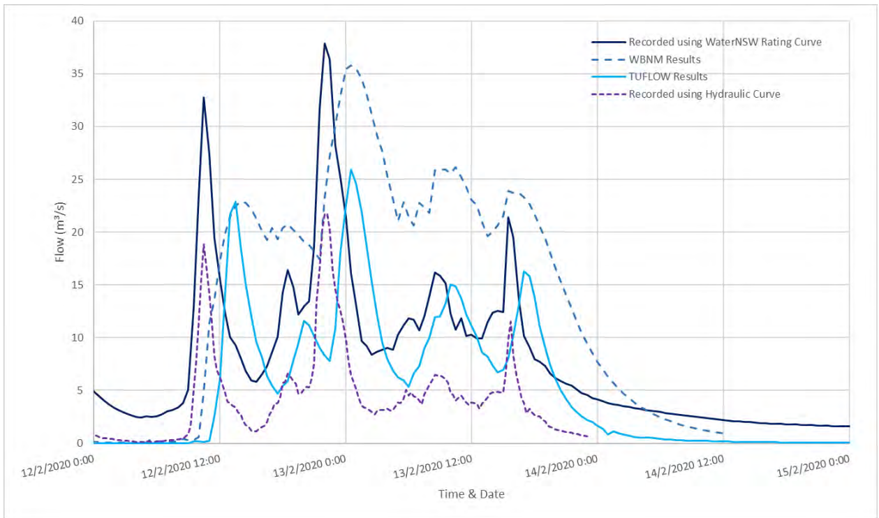
Diagram 99: 2020 Comparison of Flow at Cobaki Creek
