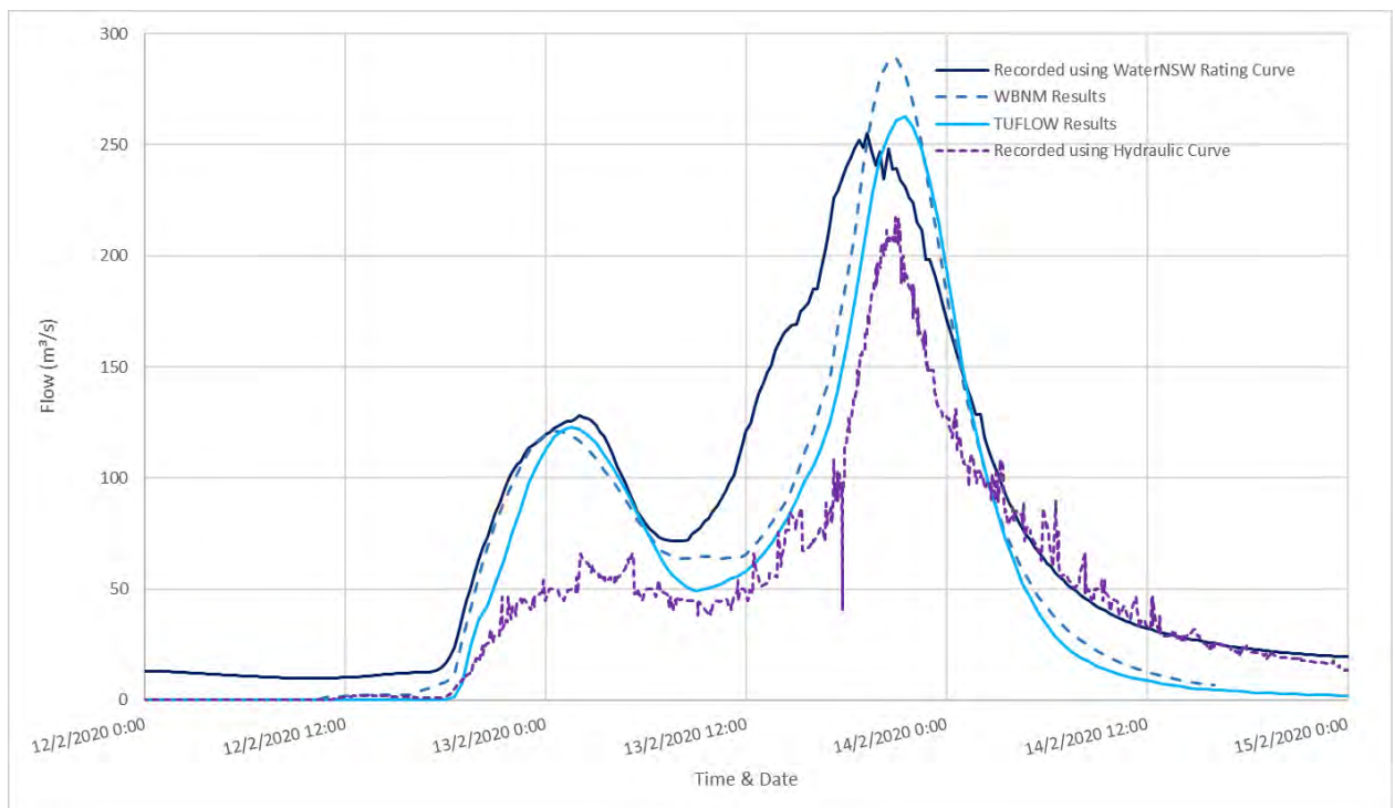
Diagram 98: 2020 Comparison of Flow at Boat Harbour
