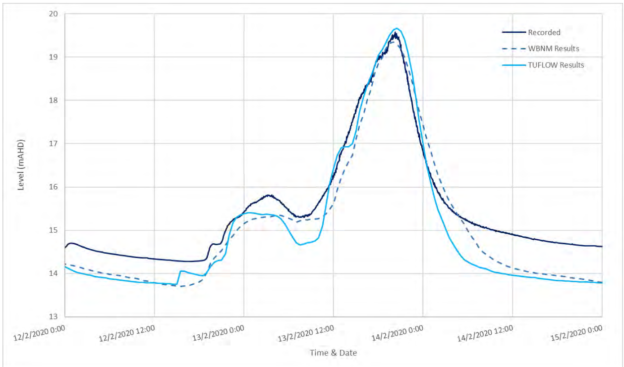
Diagram 102: 2020 Comparison of Water Level at Eungella
