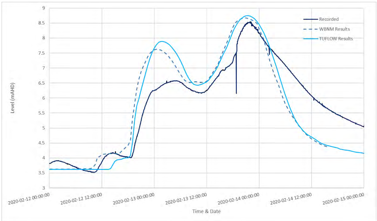
Diagram 103: 2020 Comparison of Water Level at Boat Harbour
