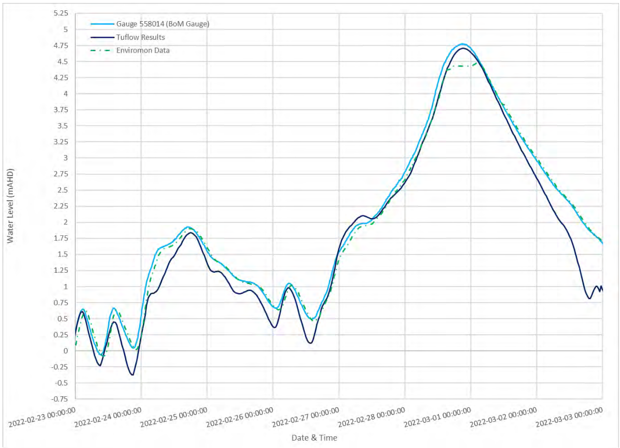
Diagram 89: 2022 Comparison of Water Level at Tumbulgum
