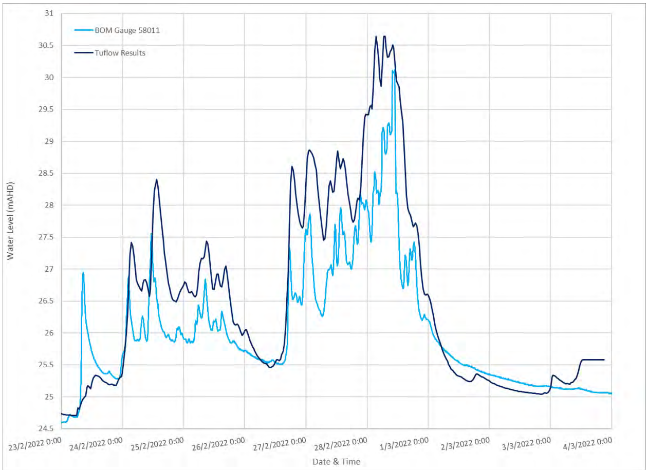
Diagram 94: 2022 Comparison of Water Level at Chillingham
