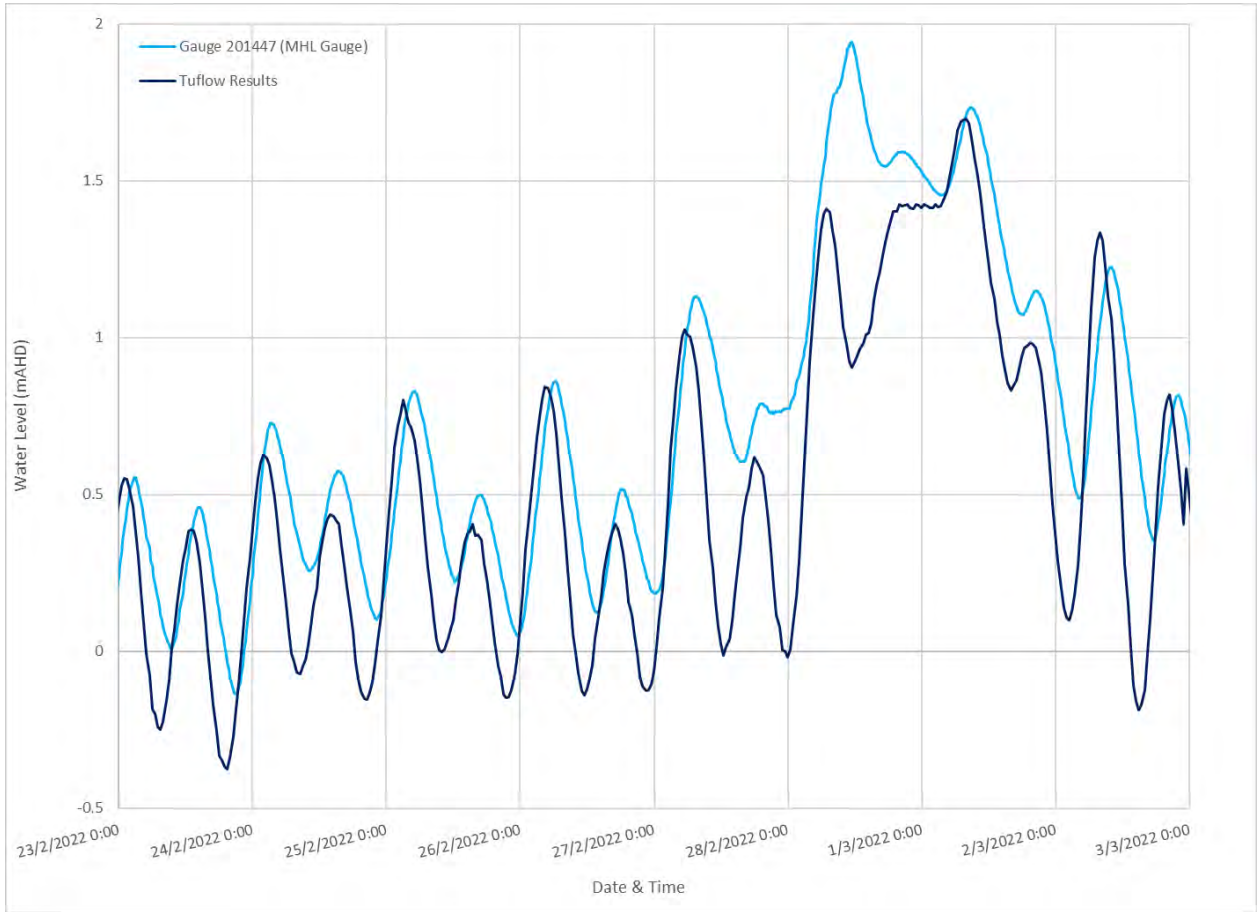
Diagram 90: 2022 Comparison of Water Level at Terranora
