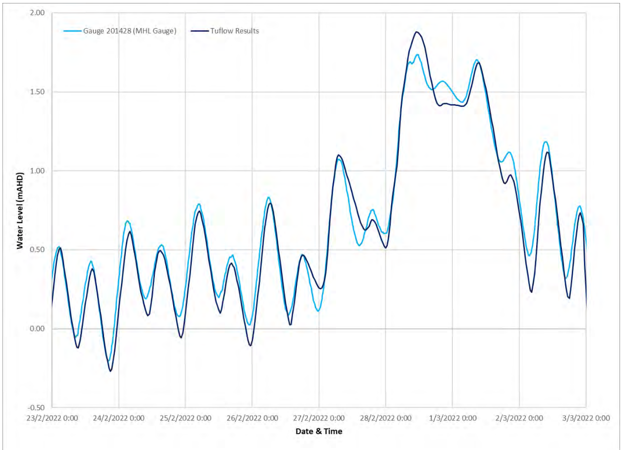
Diagram 92: 2022 Comparison of Water Level at Dry Dock
