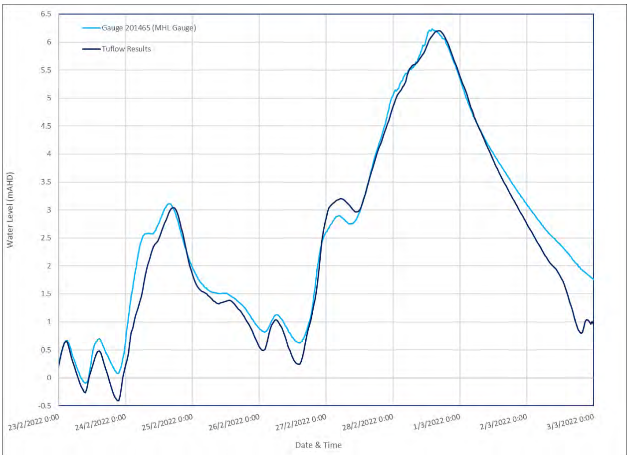
Diagram 87: 2022 Comparison of Water Level at Murwillumbah Bridge
