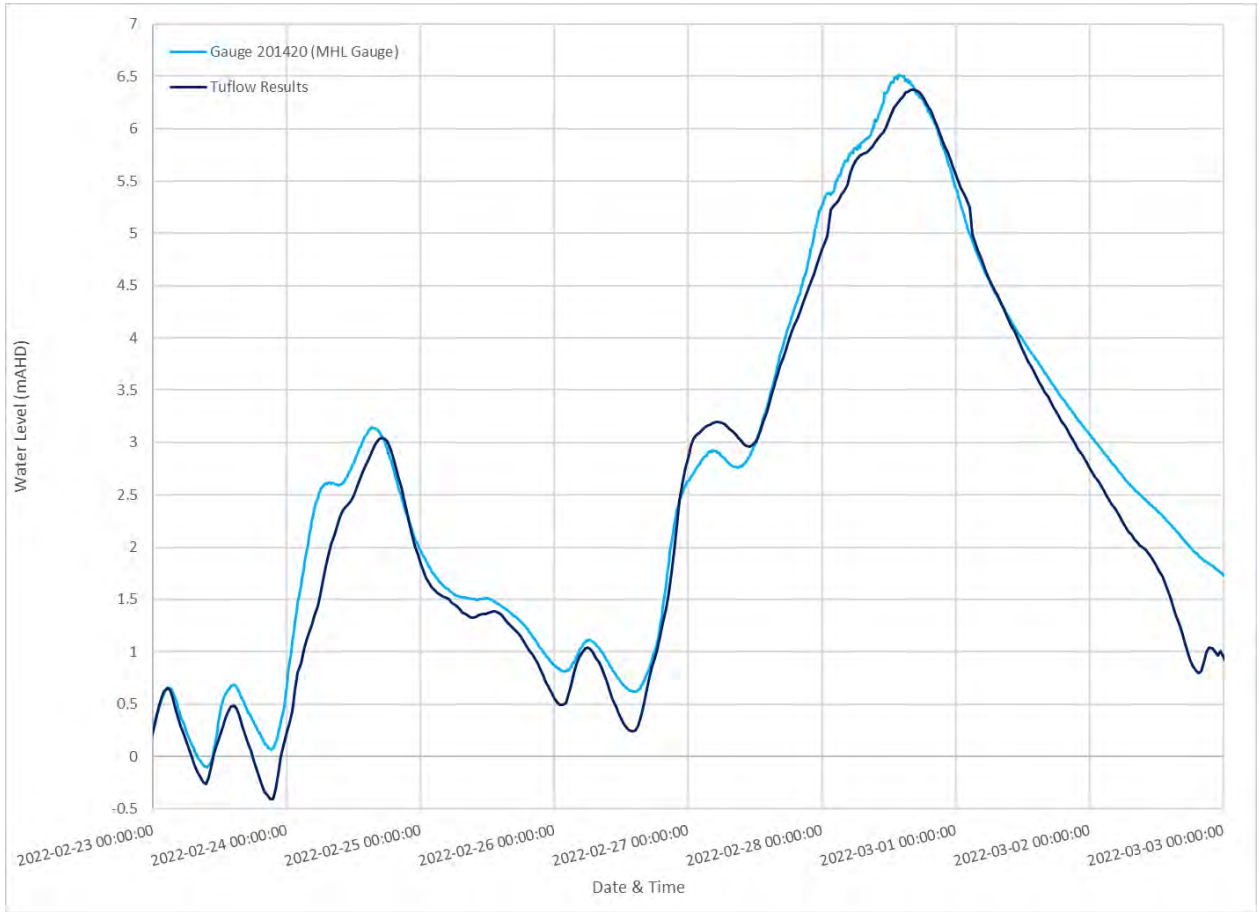
Diagram 88: 2022 Comparison of Water Level at North Murwillumbah
