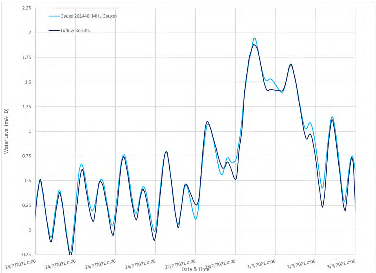
Diagram 86: 2022 Comparison of Water Level at Cobaki
