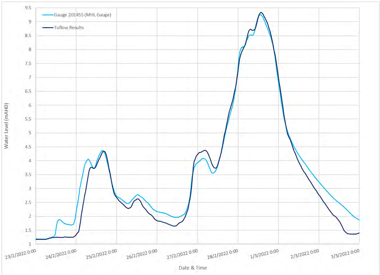
Diagram 85: 2022 Comparison of Water Level at Bray Park
