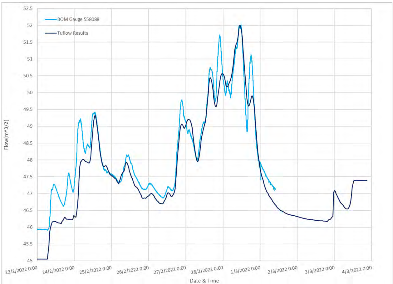
Diagram 93: 2022 Comparison of Water Level at Tyalgum Bridge
