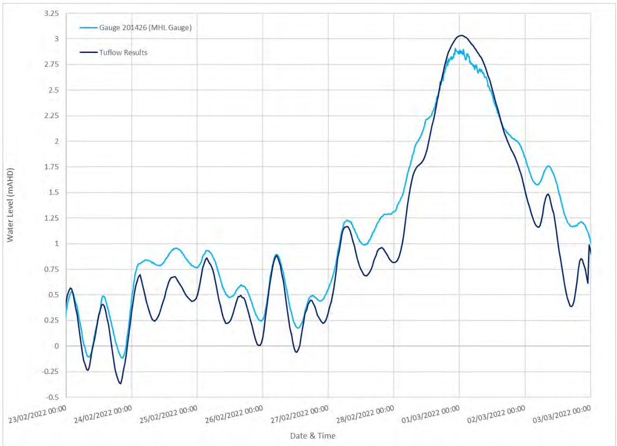
Diagram 91: 2022 Comparison of Water Level at Barney's Point
