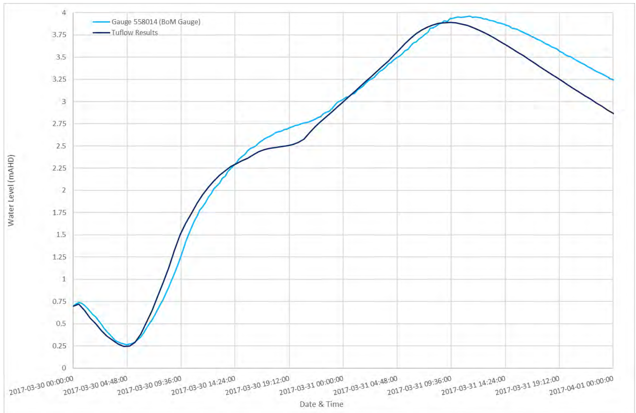
Diagram 72: 2017 Comparison of Water Level at Tumbulgum
