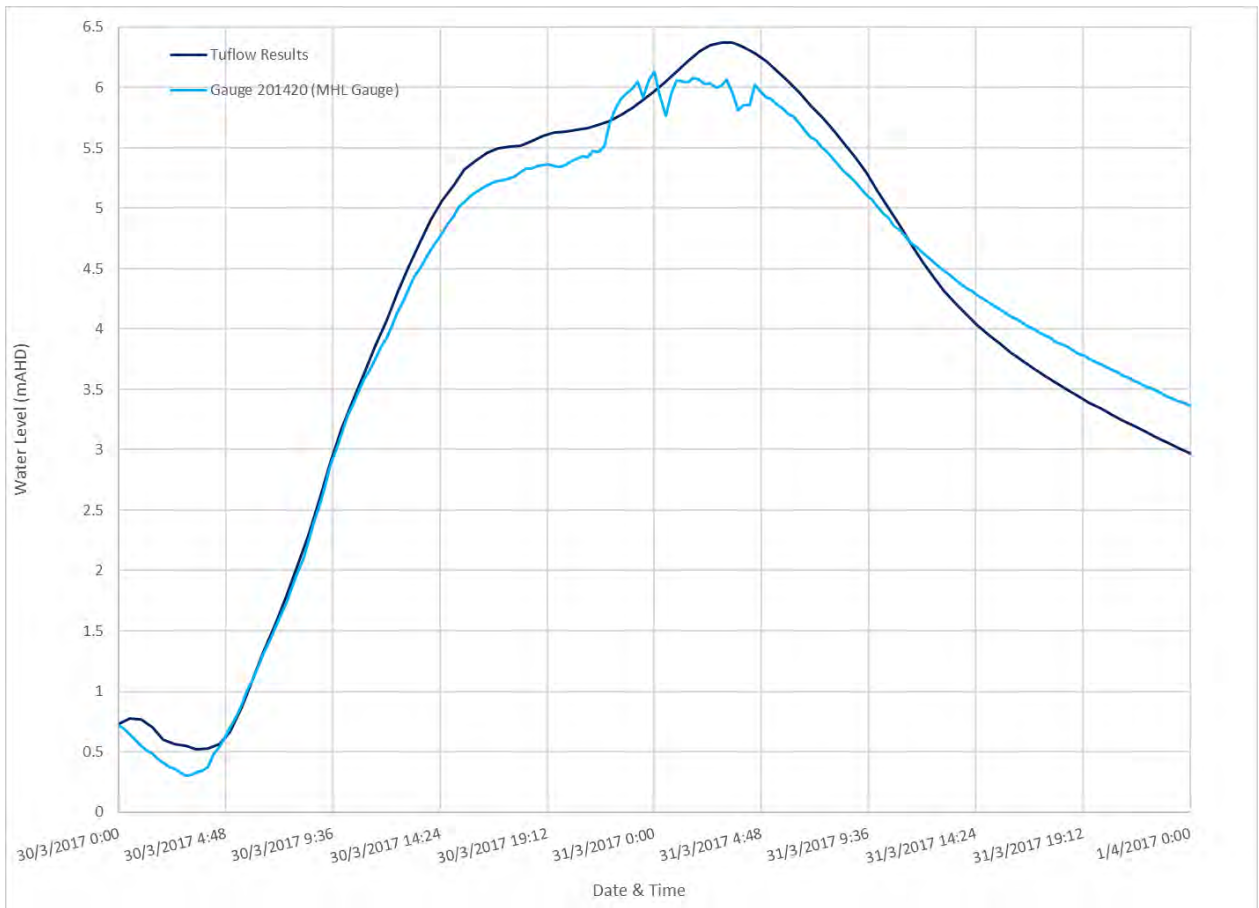
Diagram 70: 2017 Comparison of Water Level at North Murwillumbah
