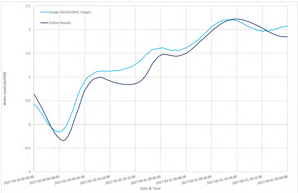
Diagram 74: 2017 Comparison of Water Level at Barney's Point
