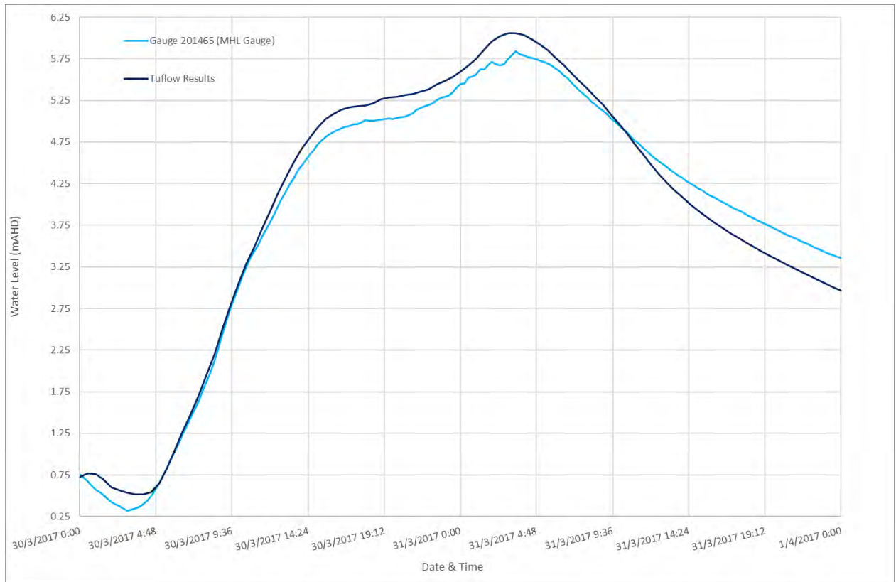
Diagram 71: 2017 Comparison of Water Level at Murwillumbah Bridge
