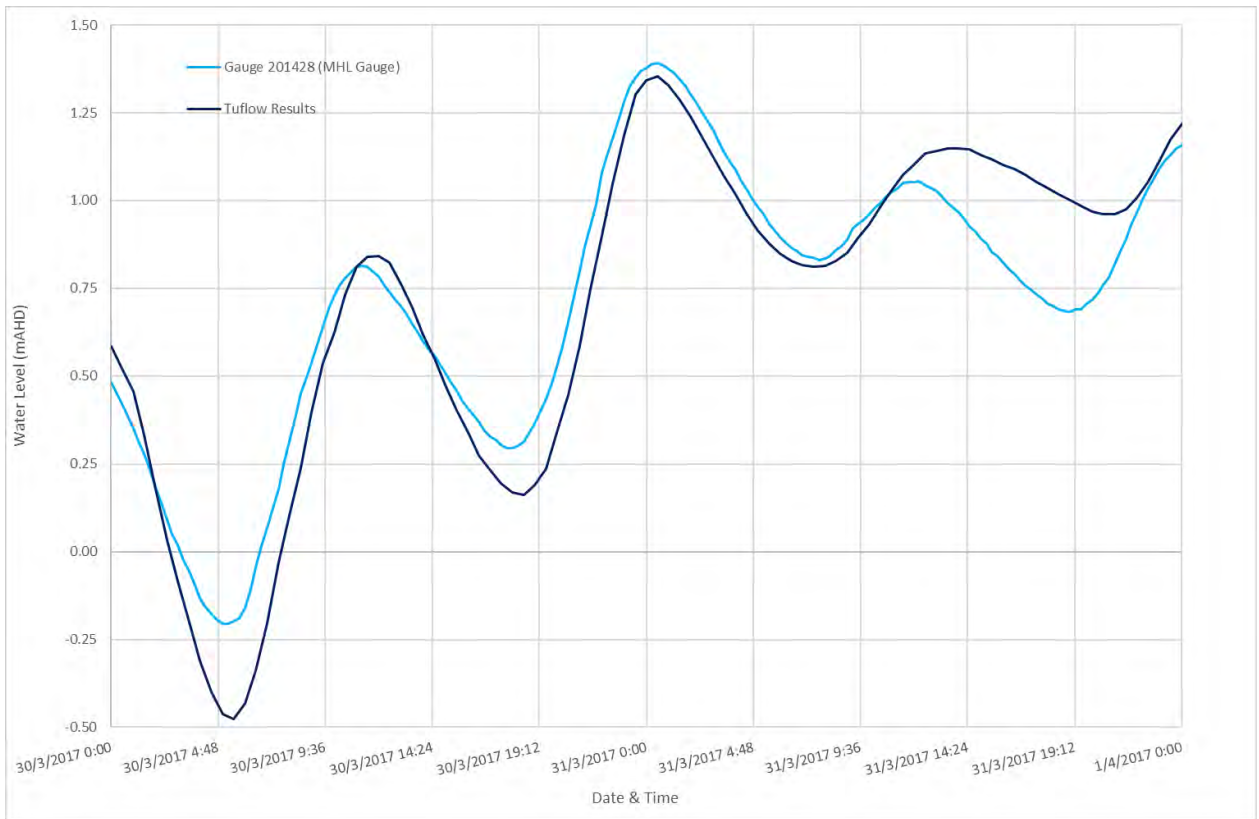
Diagram 75: 2017 Comparison of Water Level at Dry Dock
