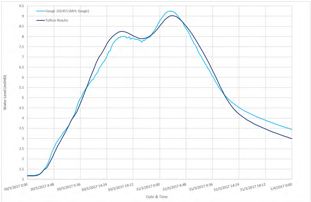
Diagram 69: 2017 Comparison of Water Level at Bray Park
