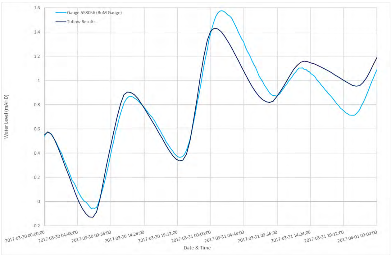
Diagram 73: 2017 Comparison of Water Level at Terranora
