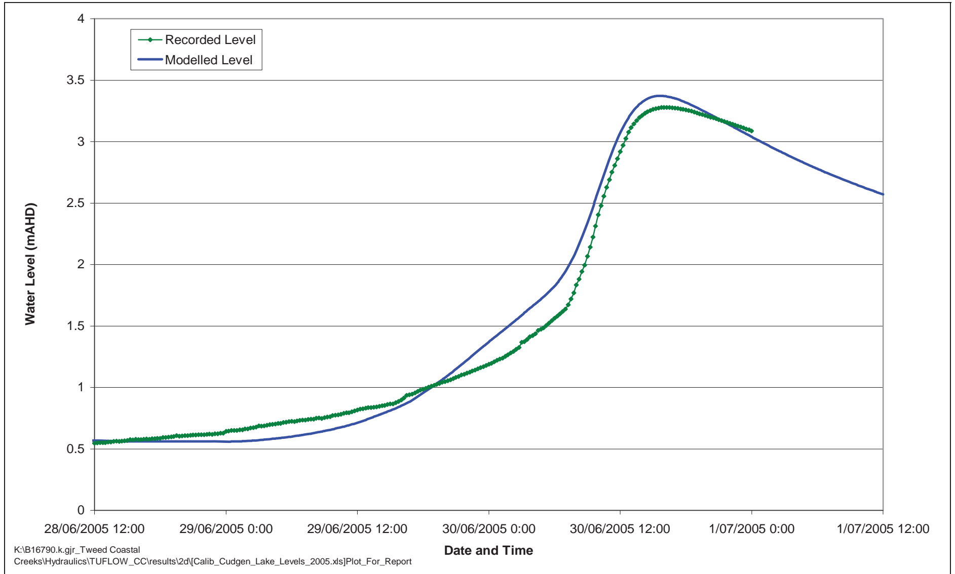
Figure 5-12 June 2005: Cudgen Lake Gauge Comparison with Hydraulic Model Results
