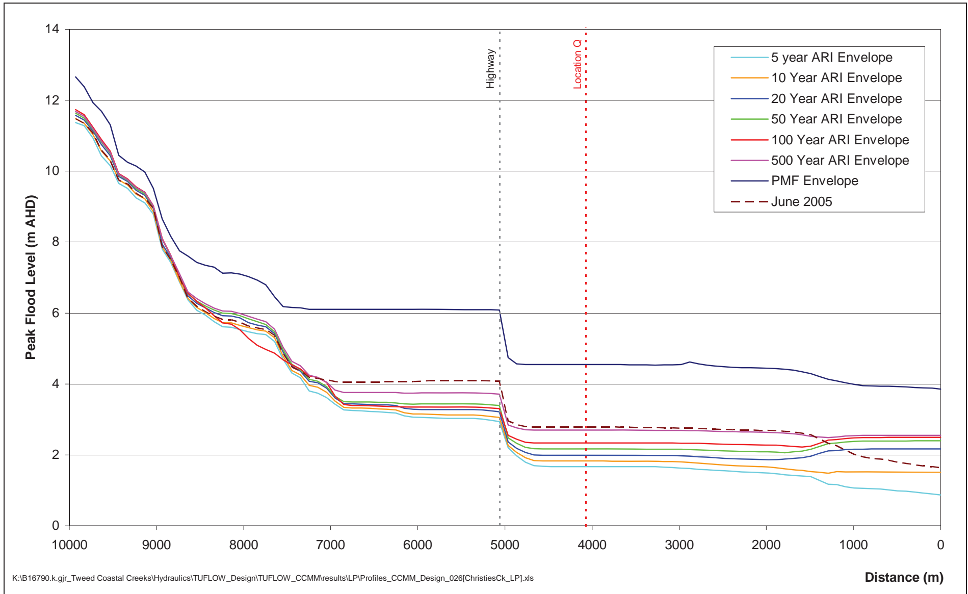
Figure 7-6 Christies Creek Flood Profile
