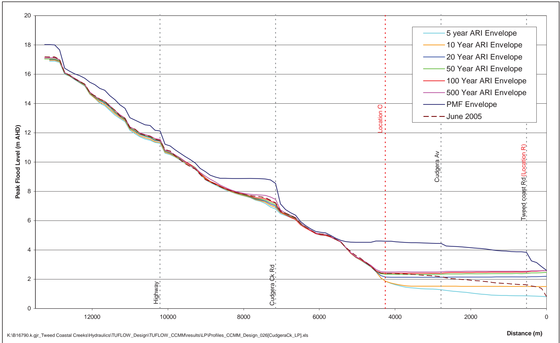
Figure 7-7 Cudgera Creek Flood Profile
