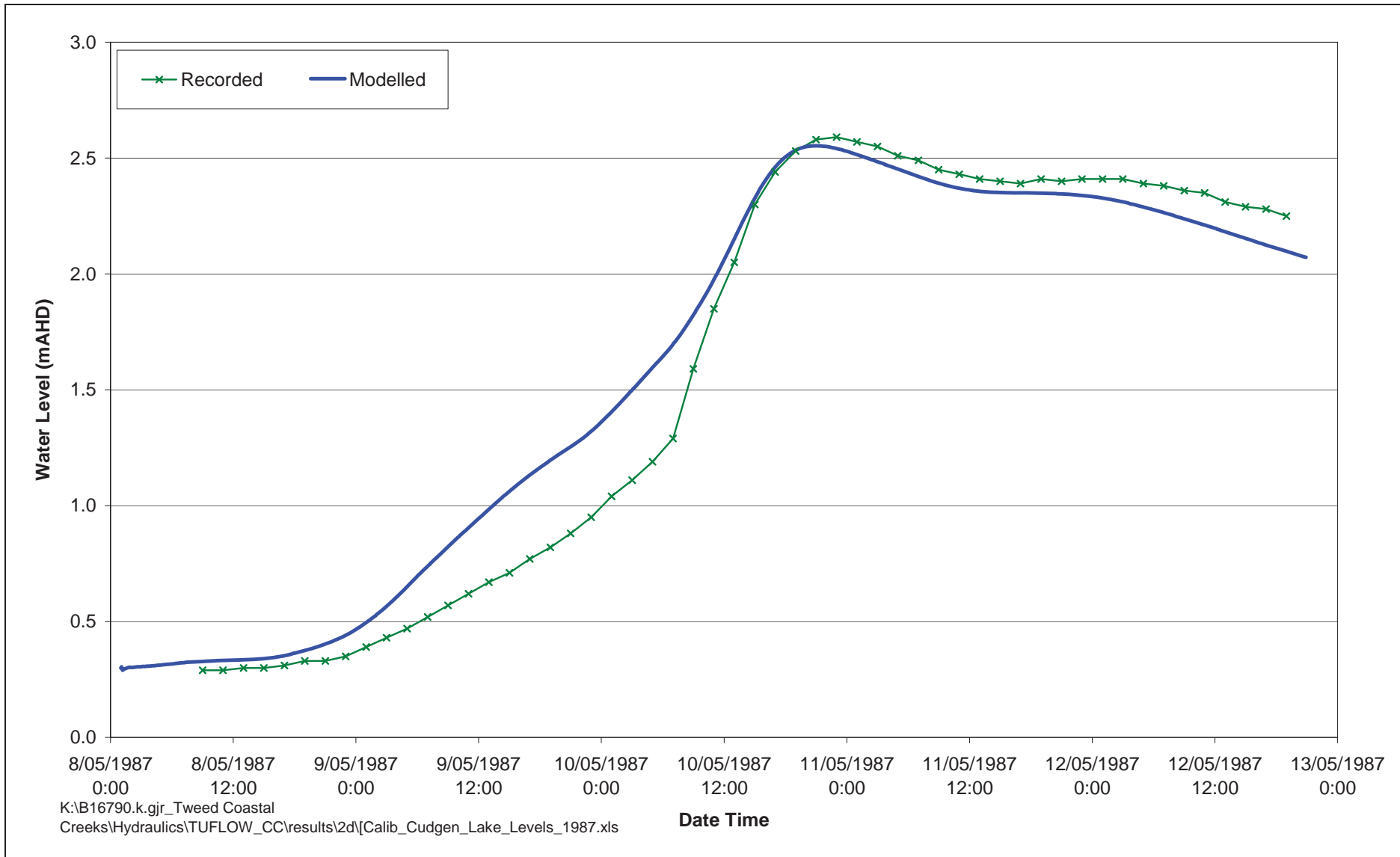
Figure 5-20 May 1987: Cudgen Lake Gauge Comparison with Hydraulic Model Results
