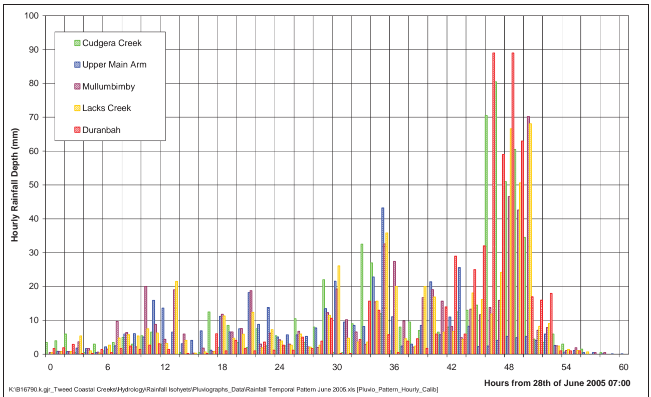
Figure 5-2 Hourly Pluviograph Patterns – June 2005 Event
