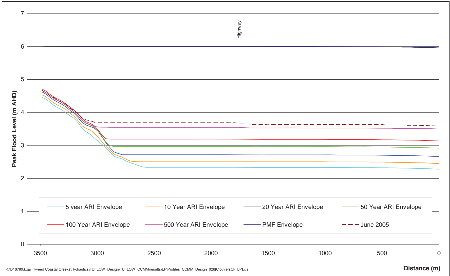
Figure 7-3 Clothiers Creek Flood Profile
