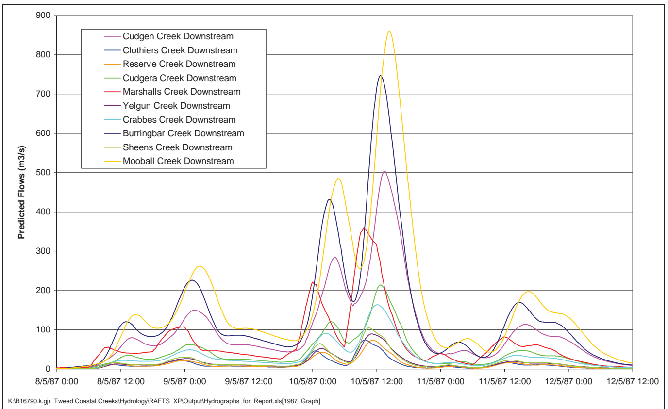
Figure 5-16 RAFTS-XP Discharge Hydrographs – May 1987 Event
