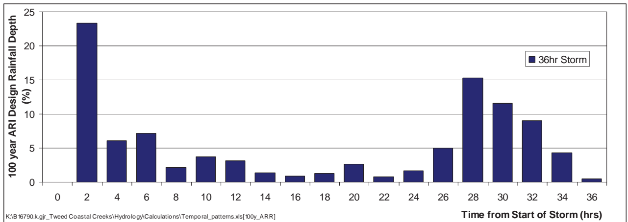
Figure 6-7 AR&R Zone 3 Temporal Pattern – 36hr Storm
