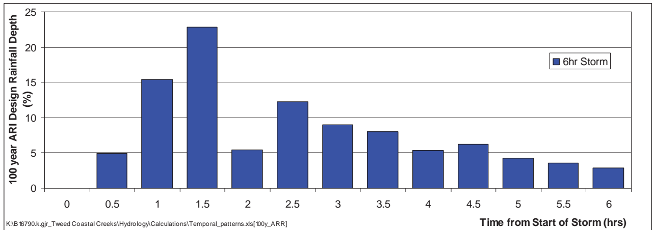
Figure 6-5 AR&R Zone 3 Temporal Pattern – 6hr Storm
