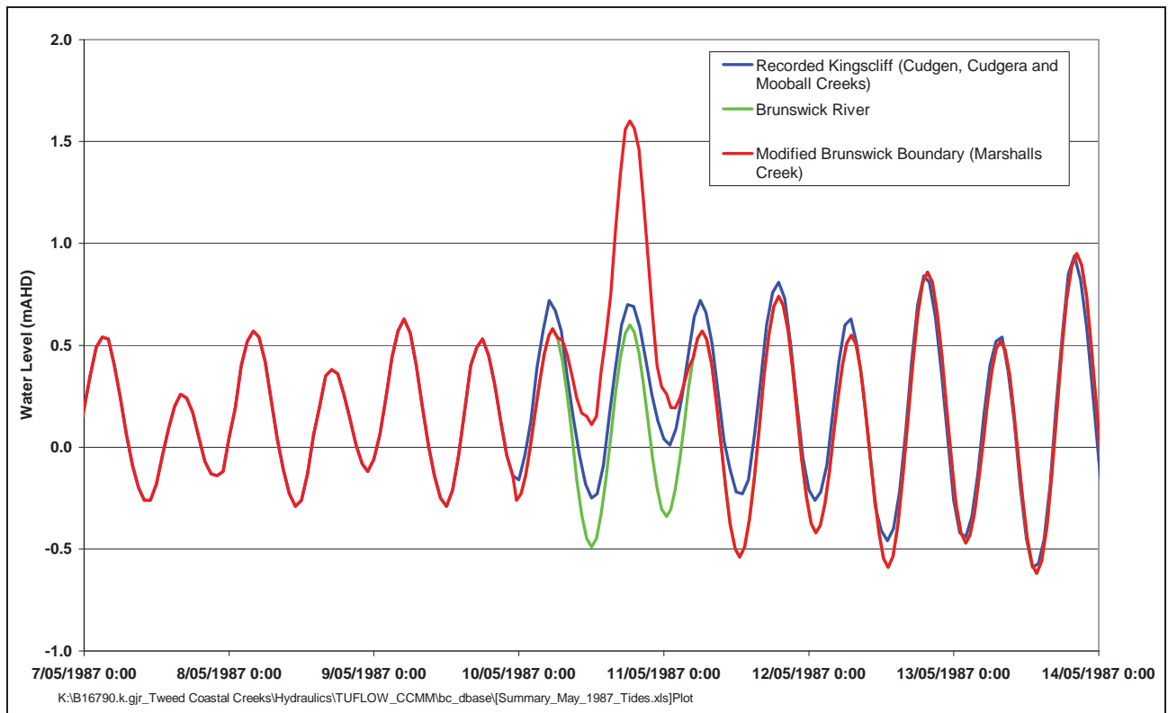
Figure 5-17 Downstream Boundary Conditions – May 1987 Event
