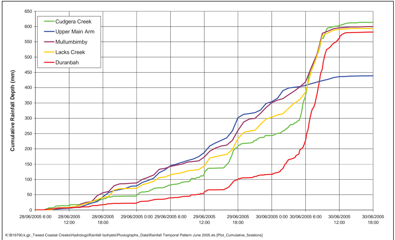
Figure 5-1 Cumulative Pluviograph Patterns – June 2005 Event
