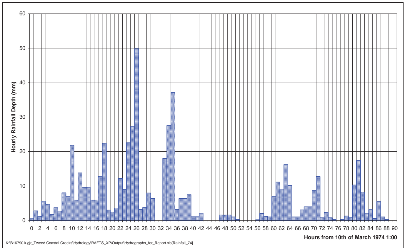
Figure 5-21 Rainfall Temporal Pattern – March 1974 Event
