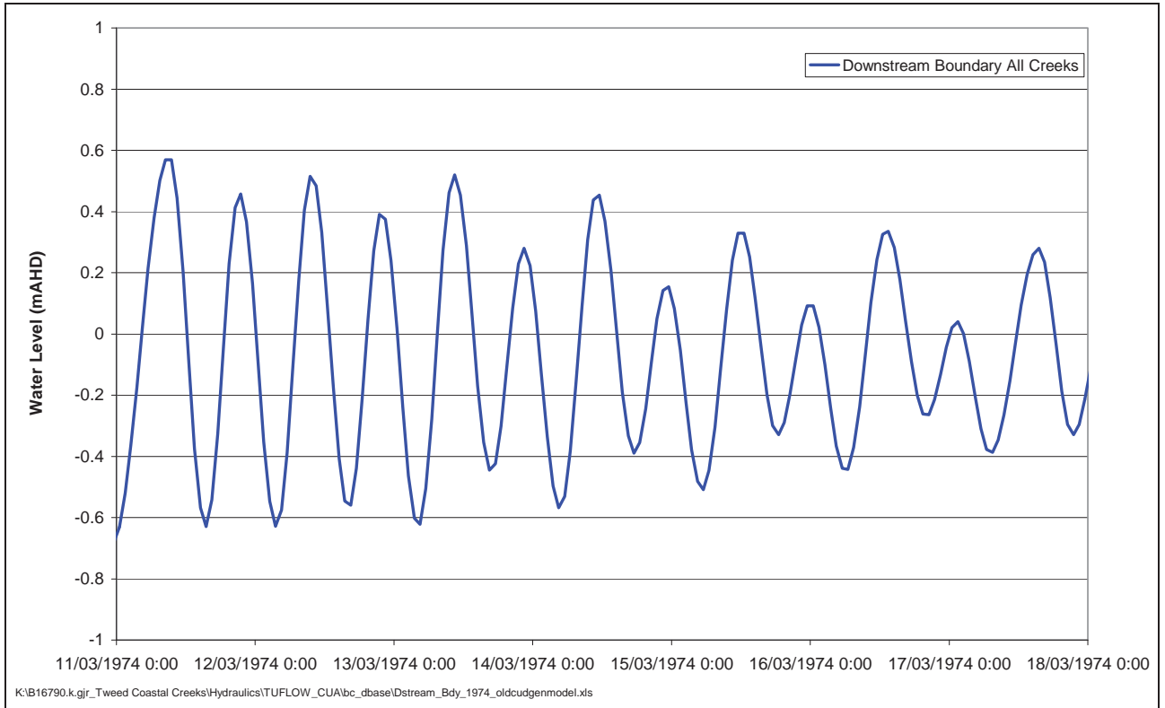
Figure 5-24 Downstream Boundary Condition – March 1974
