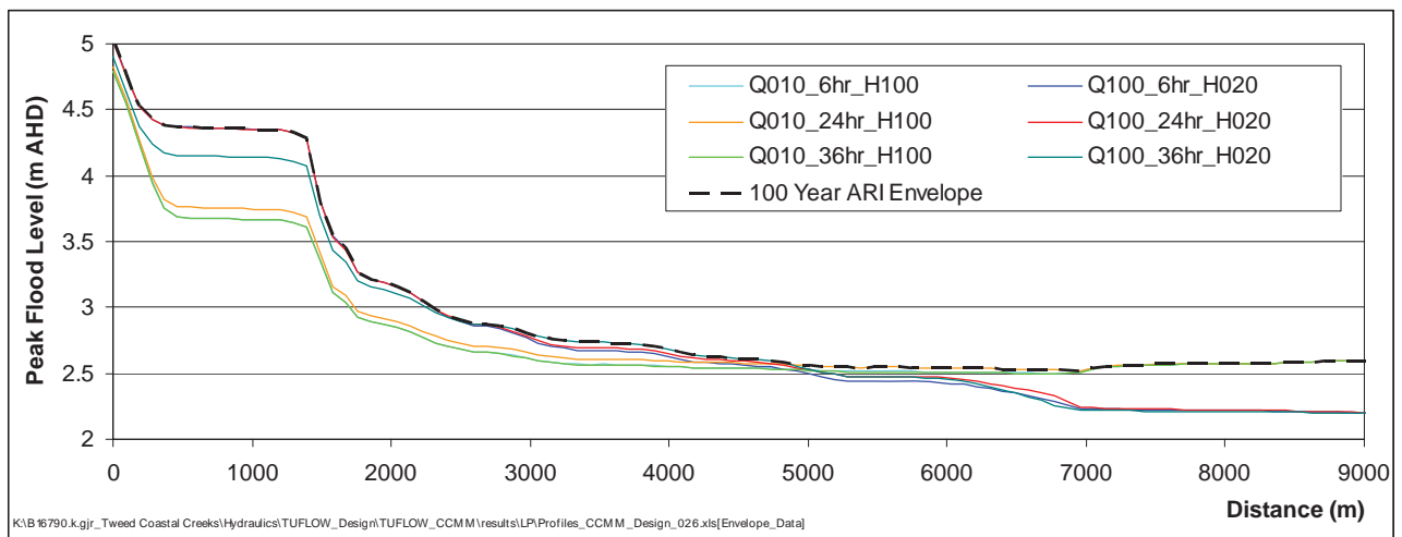
Figure 7-1 Envelope Approach Example
