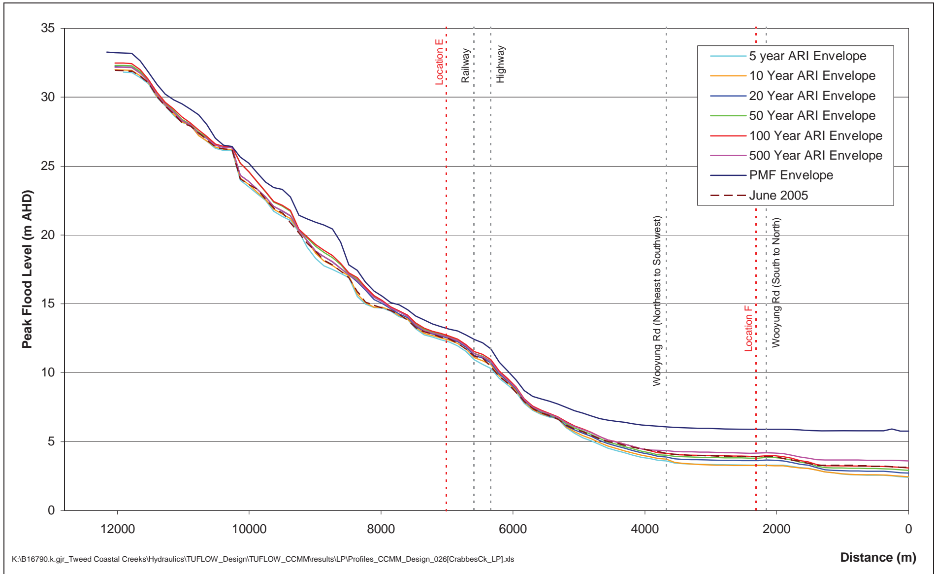
Figure 7-9 Crabbes Creek Flood Profile
