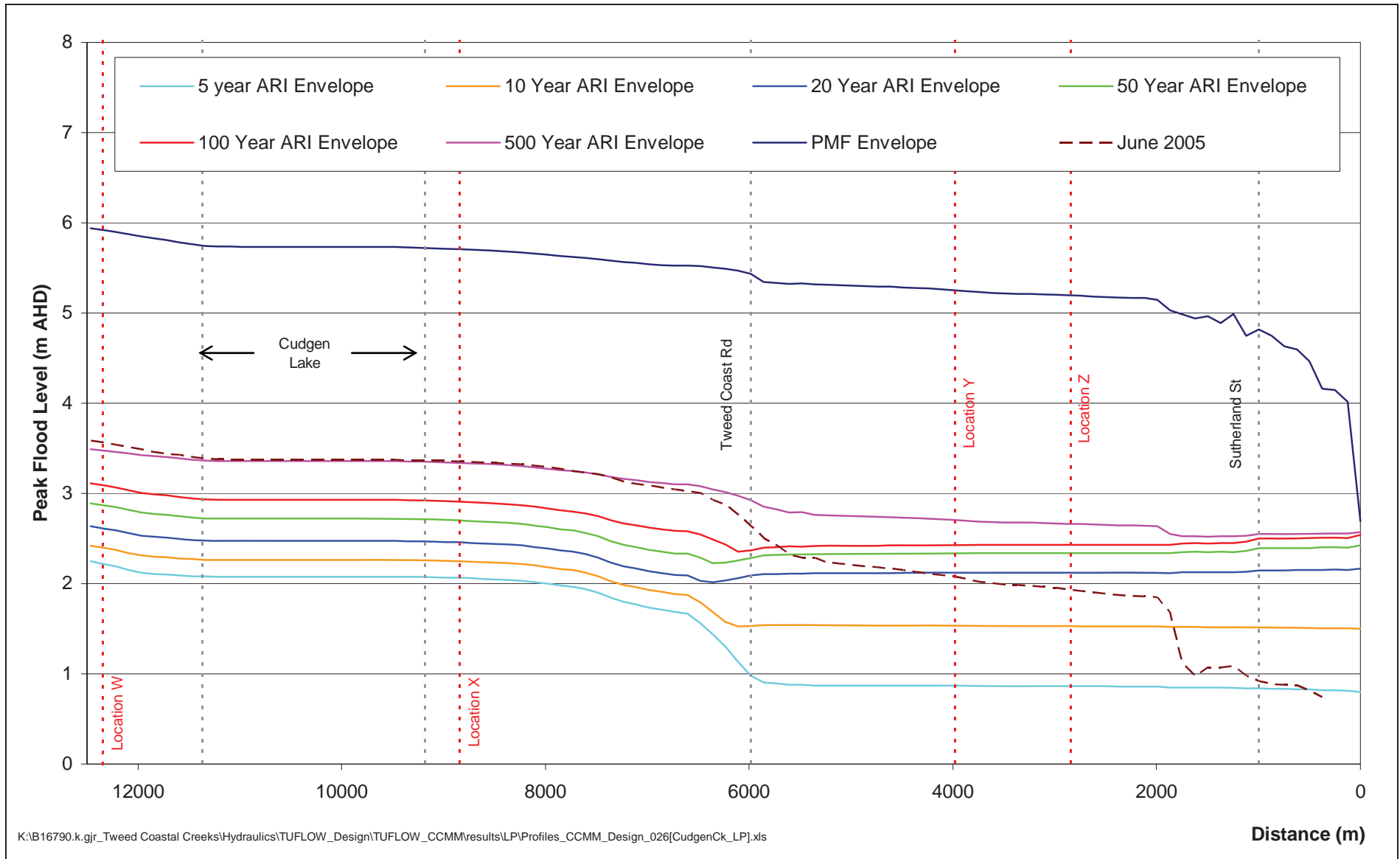
Figure 7-5 Cudgen Creek Flood Profile
