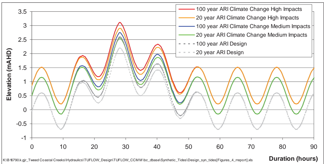
Figure 9-2 Downstream Ocean Boundary for Climate Change Scenarios – Mooball/Marshalls Creeks
