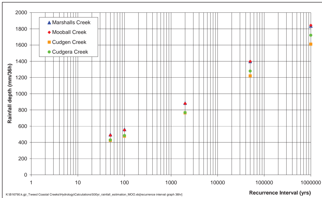
Figure 6-8 Design Rainfall Depths for a 36-hour Storm
