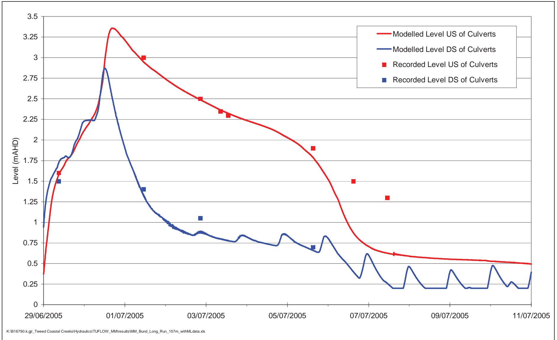
Figure 5-13 June 2005: Kallaroo Circuit Culverts Comparison with Hydraulic Model Results
