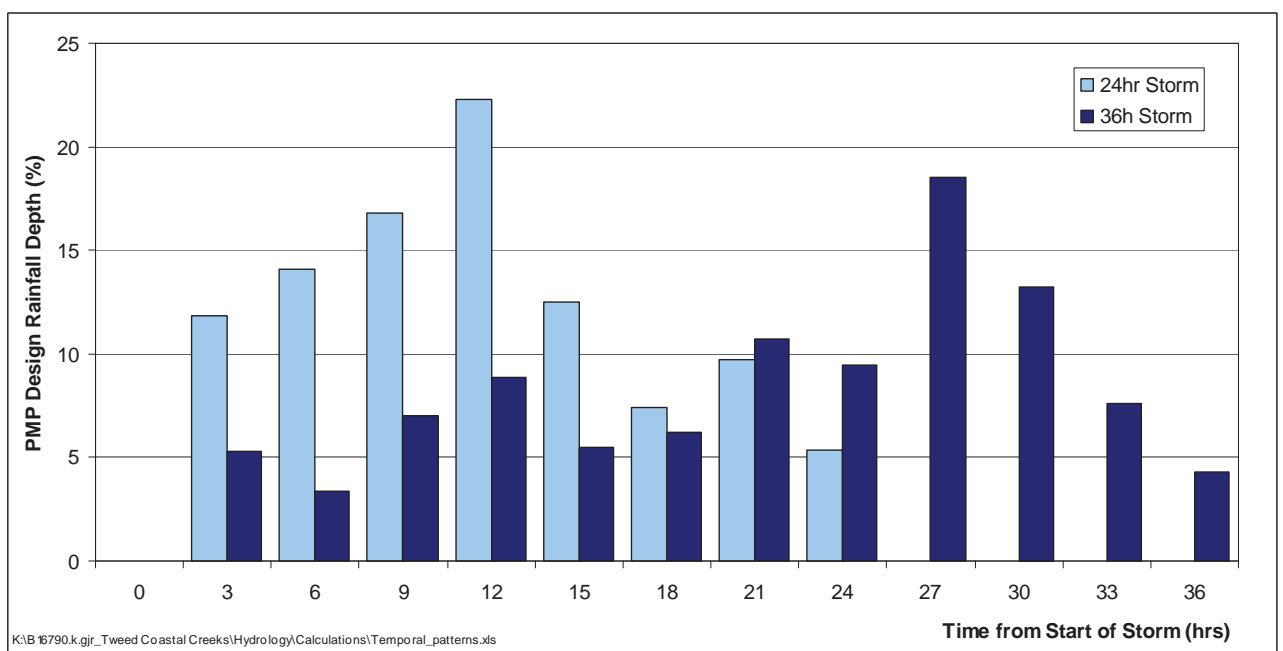
Figure 6-10 PMP Temporal Distribution – Long Duration Storm
