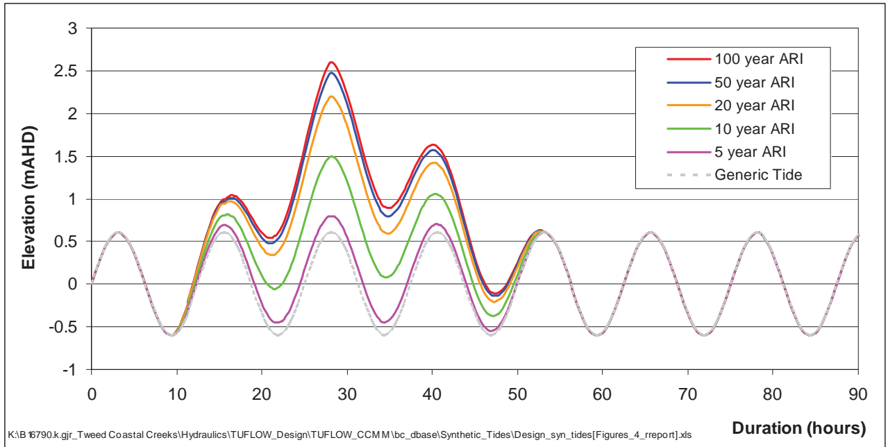
Figure 6-12 Downstream Ocean Boundary for Design Events – Cudgen/Cudgera Creeks
