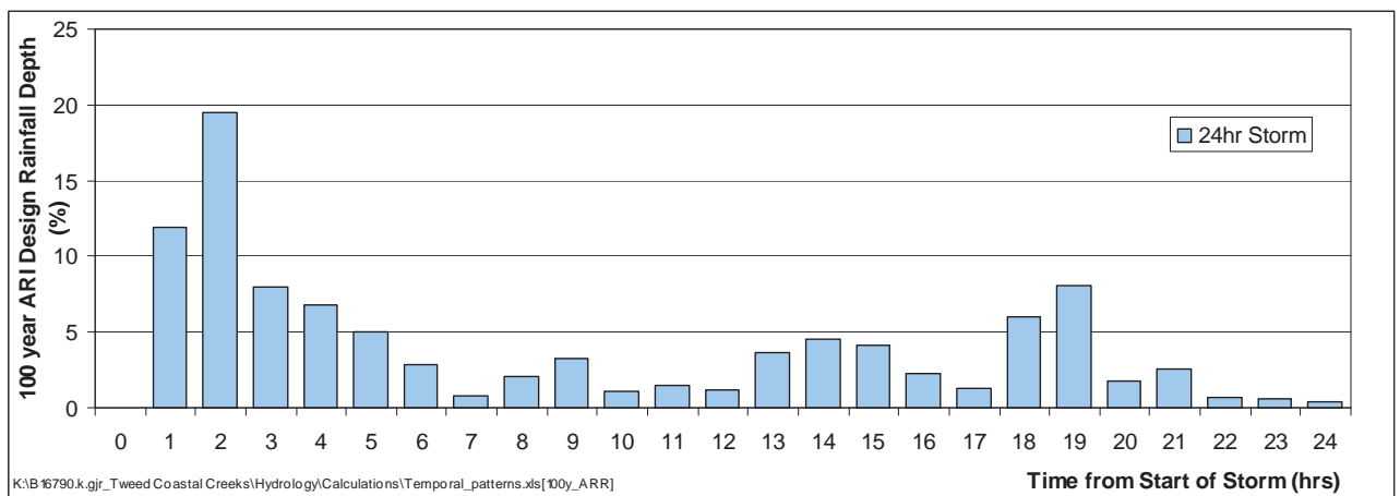
Figure 6-6 AR&R Zone 3 Temporal Pattern – 24hr Storm
