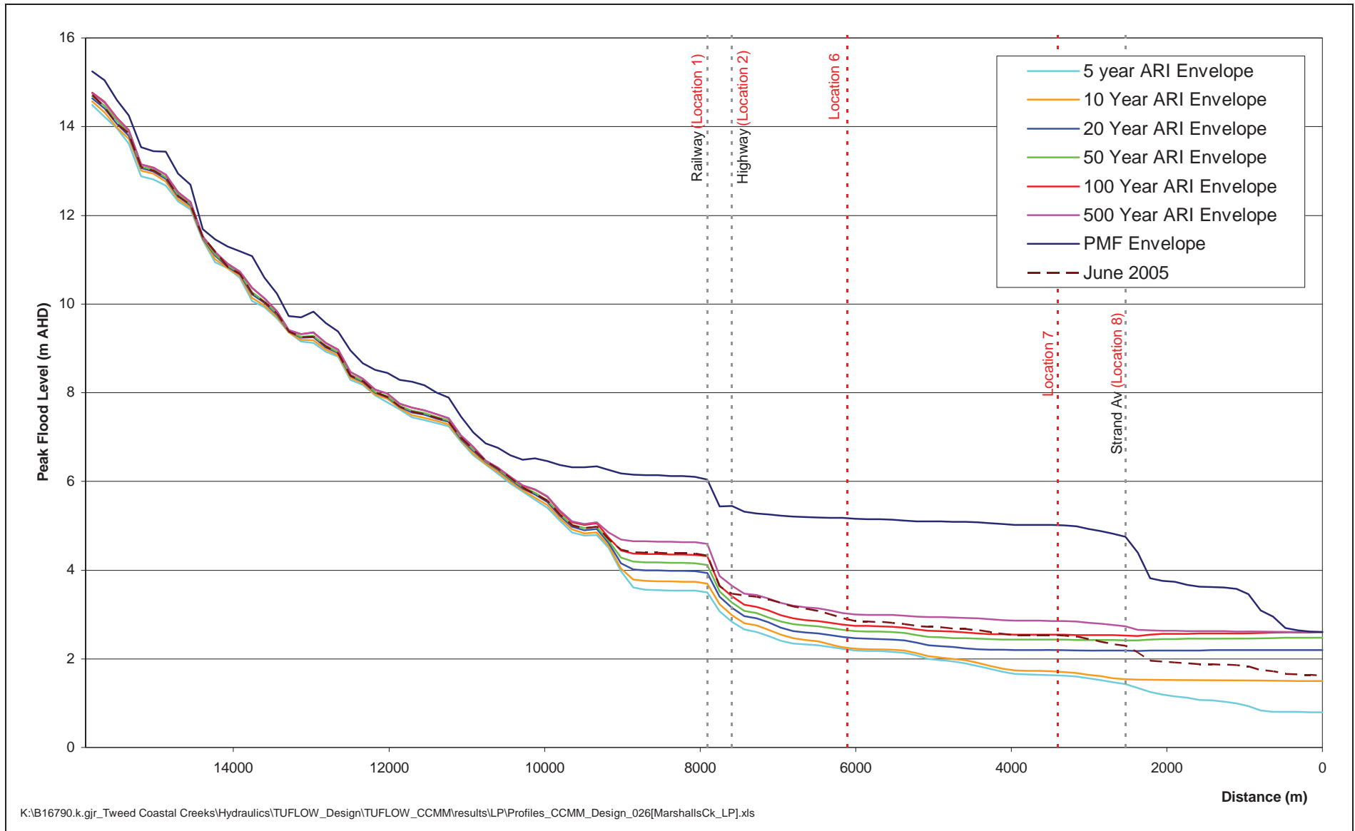
Figure 7-11 Marshalls Creek Flood Profile
