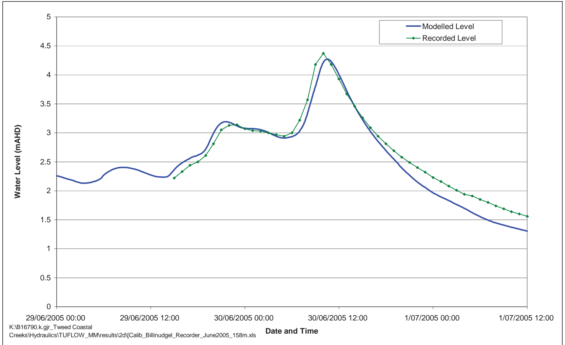
Figure 5-11 June 2005: Billinudgel Gauge Comparison with Hydraulic Model Results
