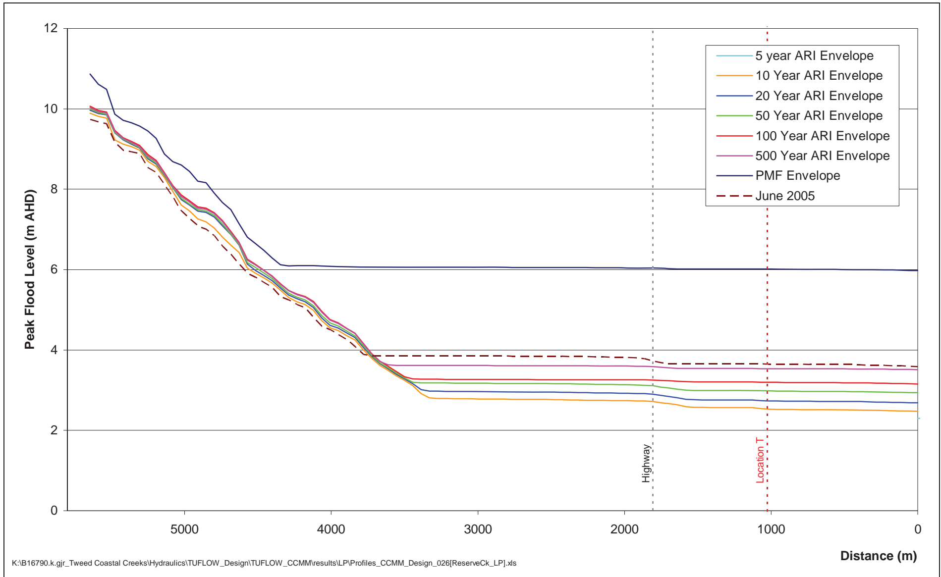
Figure 7-4 Reserve Creek Flood Profile
