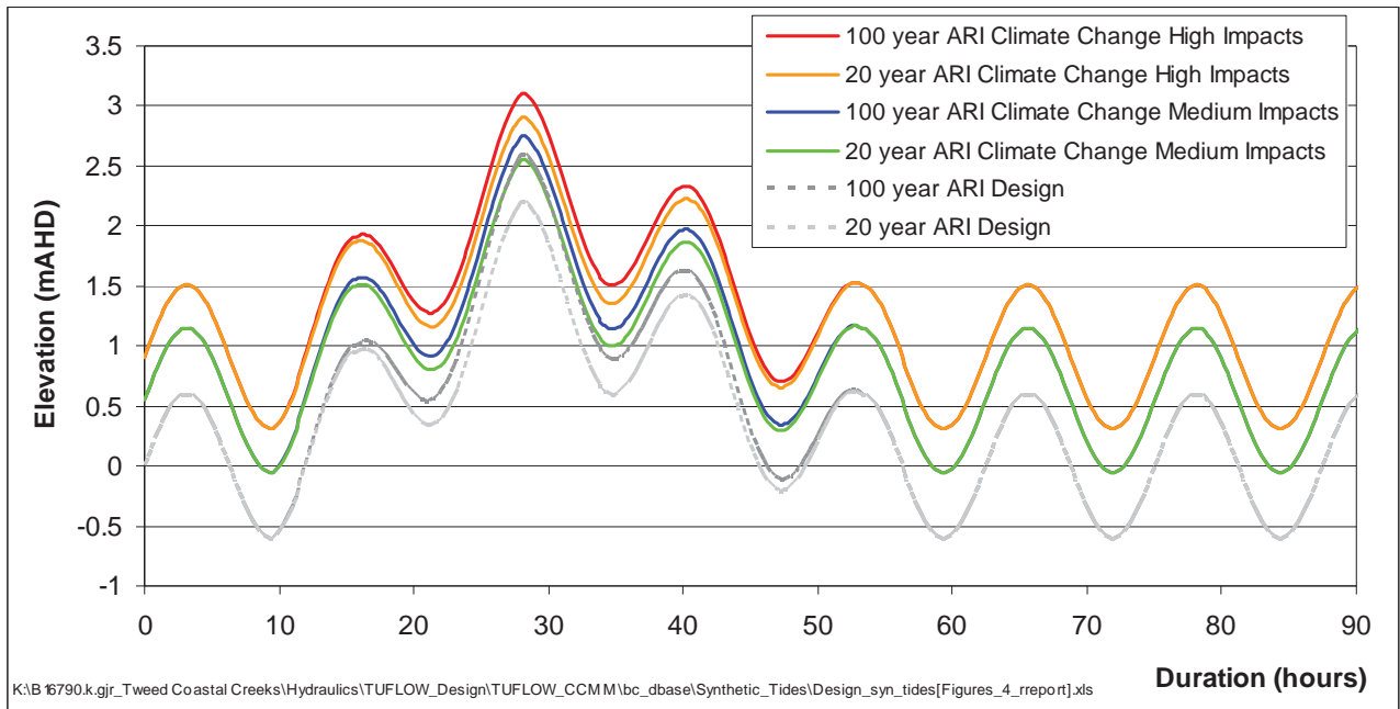
Figure 9-1 Downstream Ocean Boundary for Climate Change Scenarios – Cudgen/Cudgera Creeks
