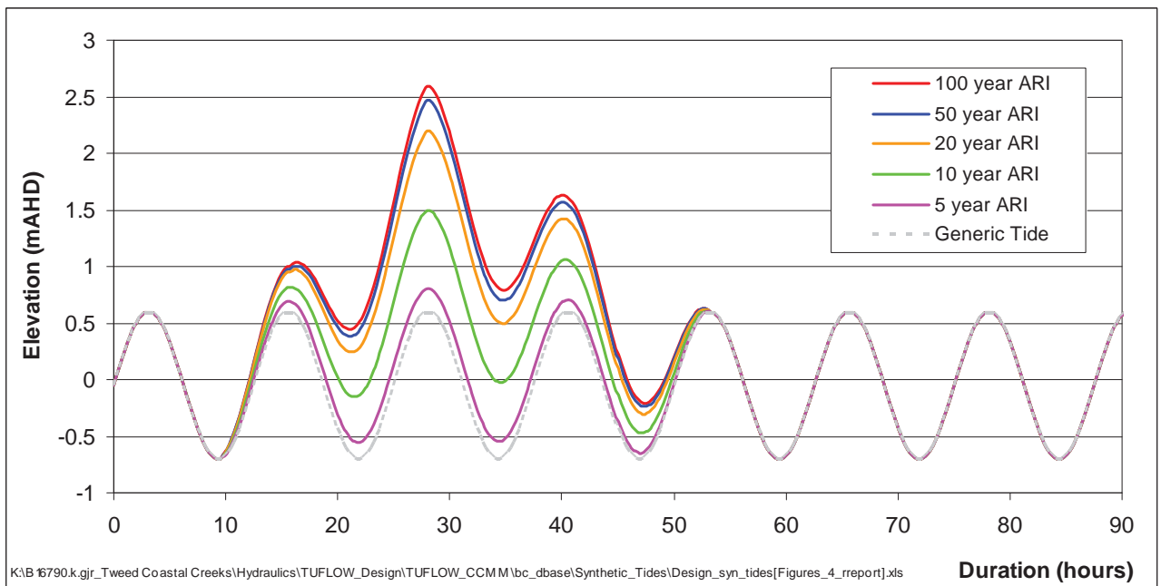
Figure 6-13 Downstream Ocean Boundary for Design Events – Mooball/Marshalls Creeks
