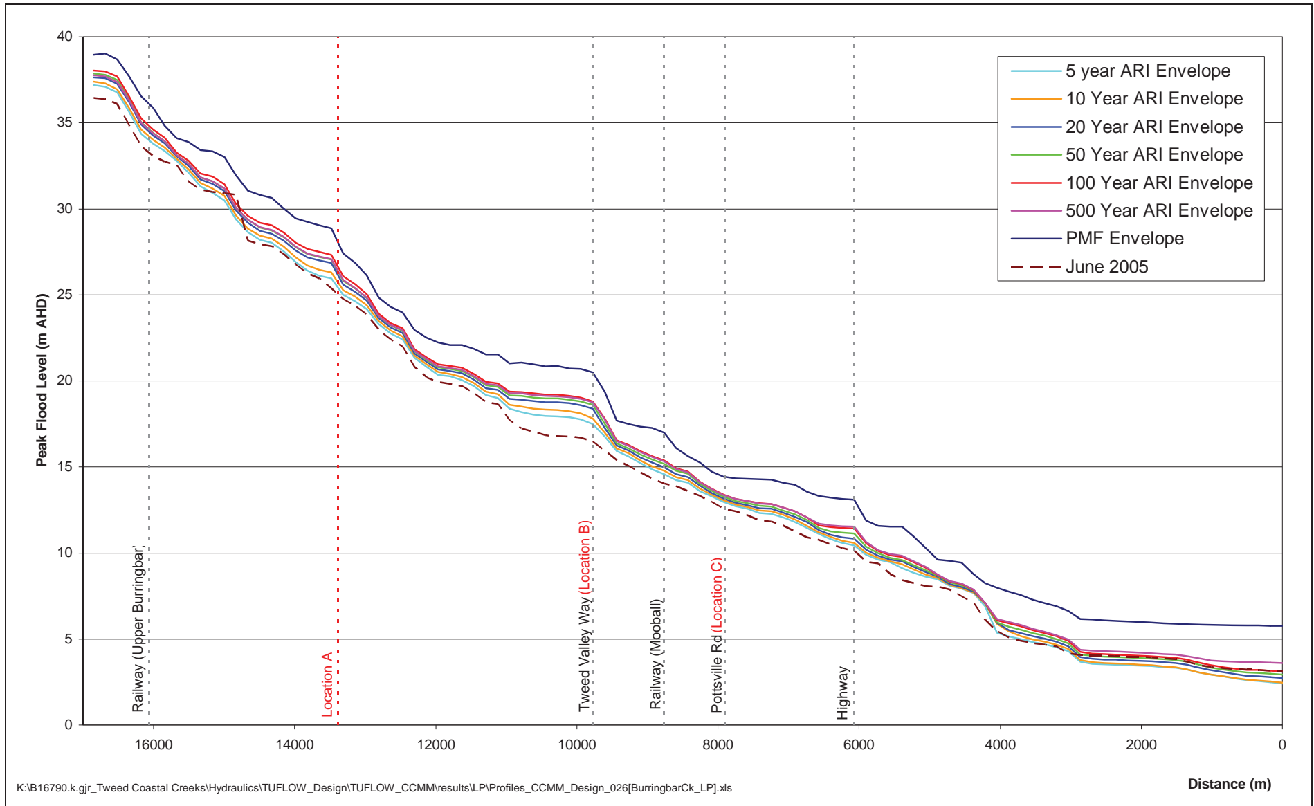
Figure 7-8 Burringbar Creek Flood Profile
