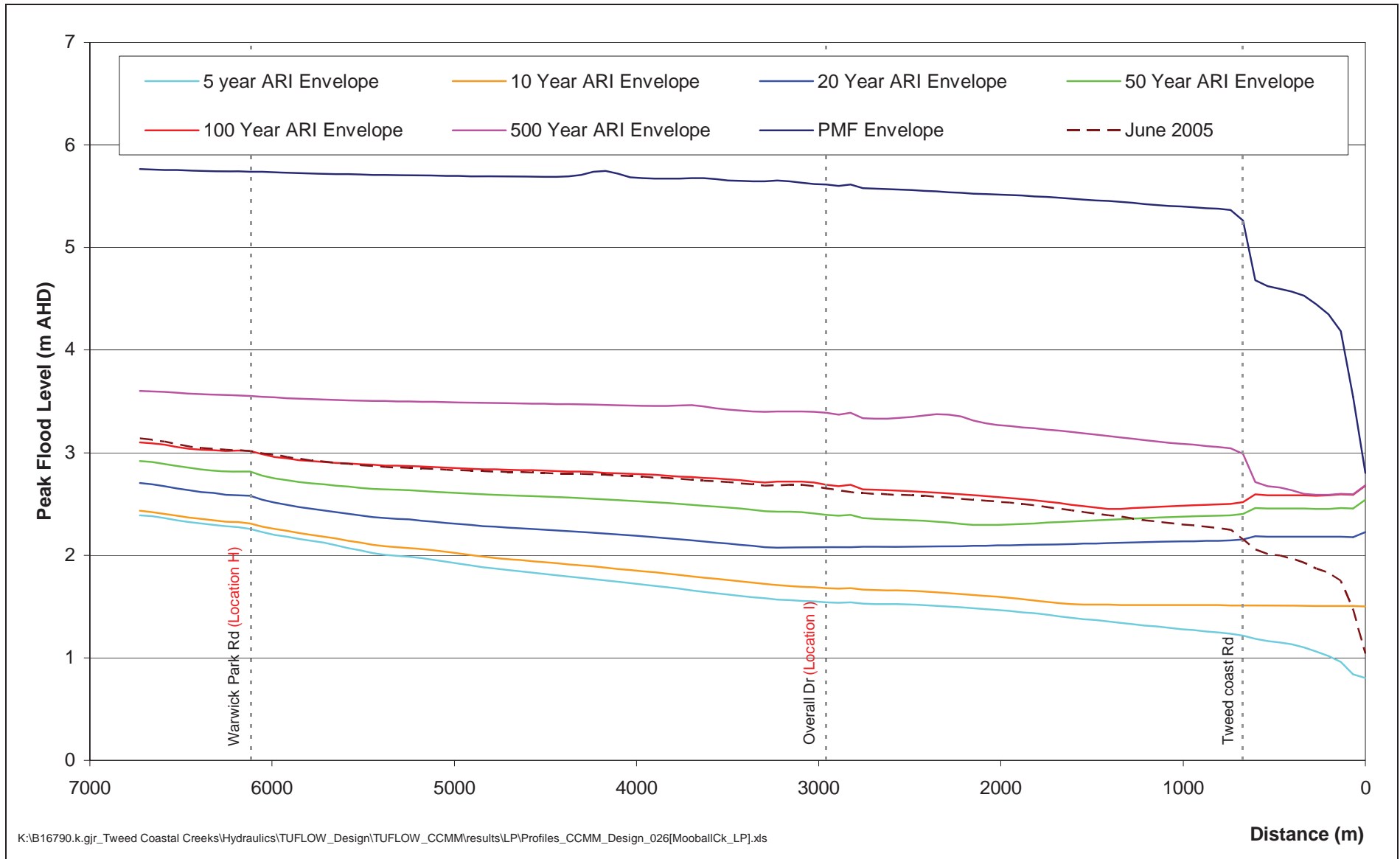
Figure 7-10 Mooball Creek Flood Profile
