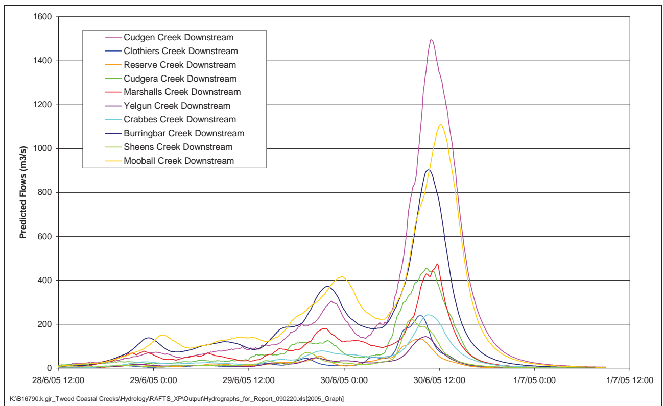
Figure 5-7 RAFTS-XP Discharge Hydrographs – June 2005 Event
