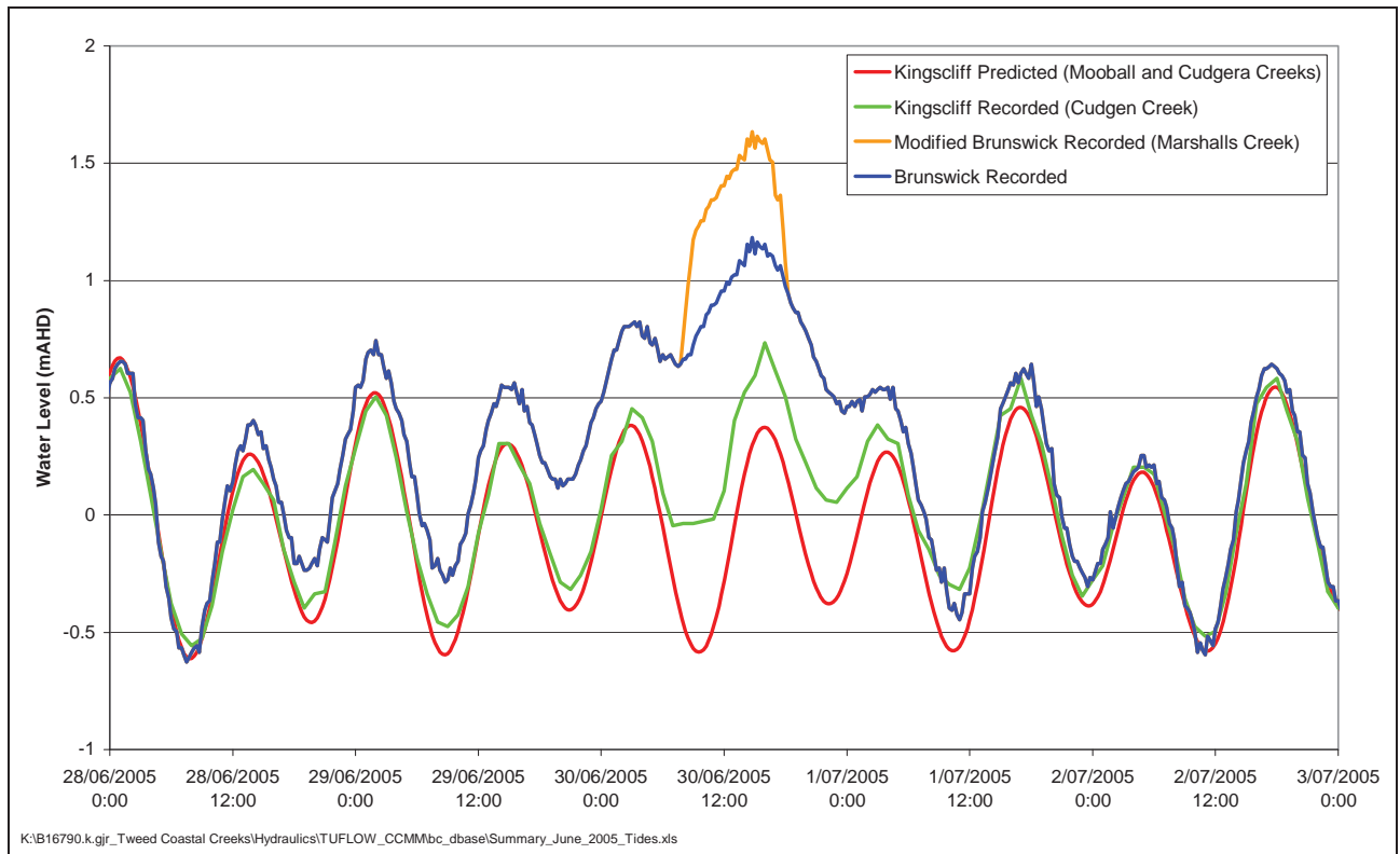
Figure 5-8 Downstream Boundary Conditions – June 2005 Event
