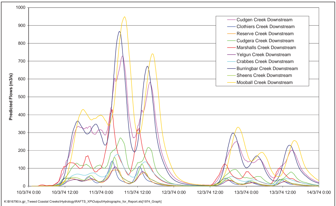
Figure 5-23 RAFTS-XP Discharge Hydrographs – March 1974 Event
