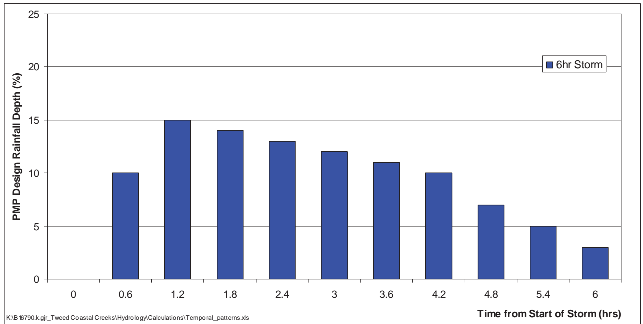
Figure 6-9 PMP Temporal Distribution – Short Duration Storm
