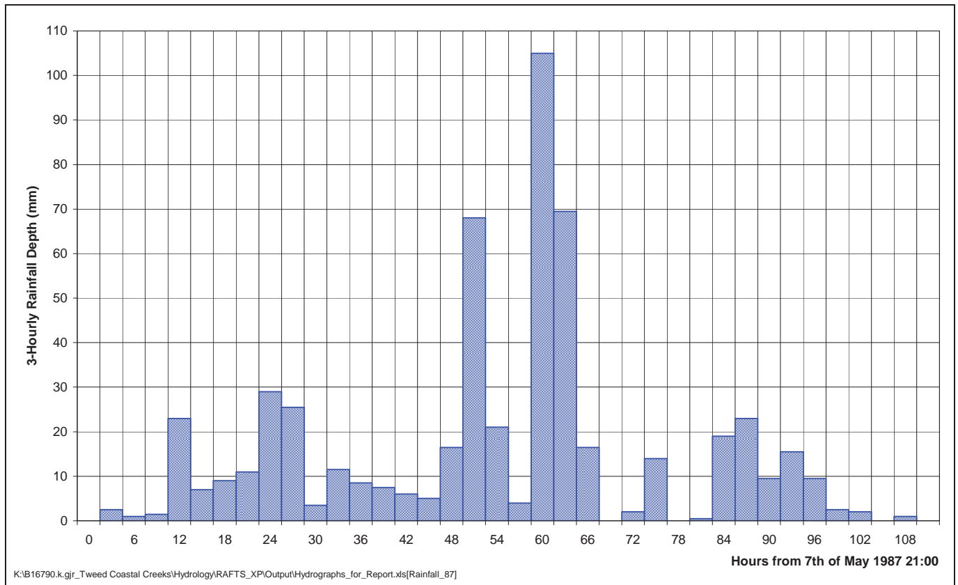
Figure 5-14 Rainfall Temporal Pattern – May 1987 Event
