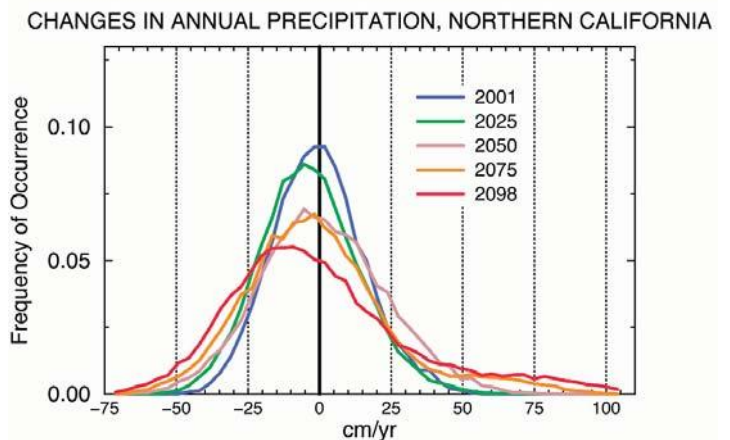
Figure 4. Time slices of the distributions of resampled ensemble realizations in Figure 3.
