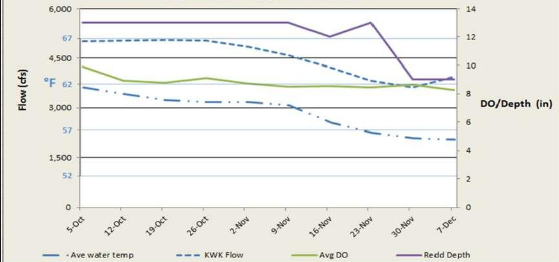
Average Weekly DO, Temperature, Flows and Water Depth by Date Sacramento River Mile 292: inside Redd #1079
