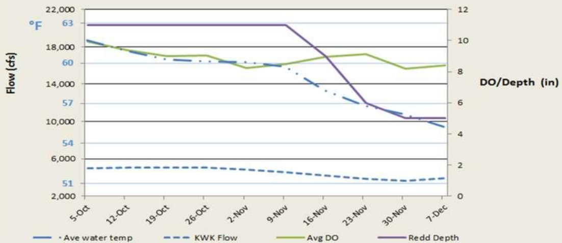
Average Weekly DO, Temperature, Flows and Water Depth by Date Sacramento River Mile 292: inside Redd #1081
