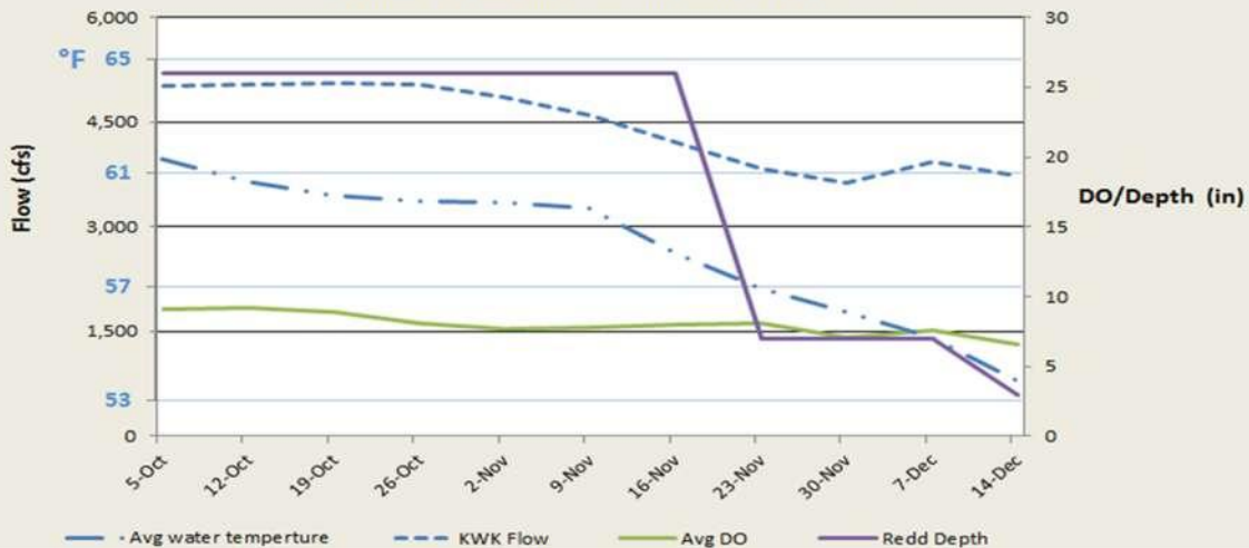
Average Weekly DO, Temperature, Flows and Water Depth by Date Sacramento River Mile 296: inside Redd #1069
