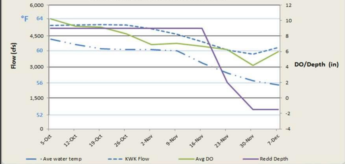
Average Weekly DO, Temperature, Flows and Water Depth by Date Sacramento River Mile 297: inside Redd #1073
