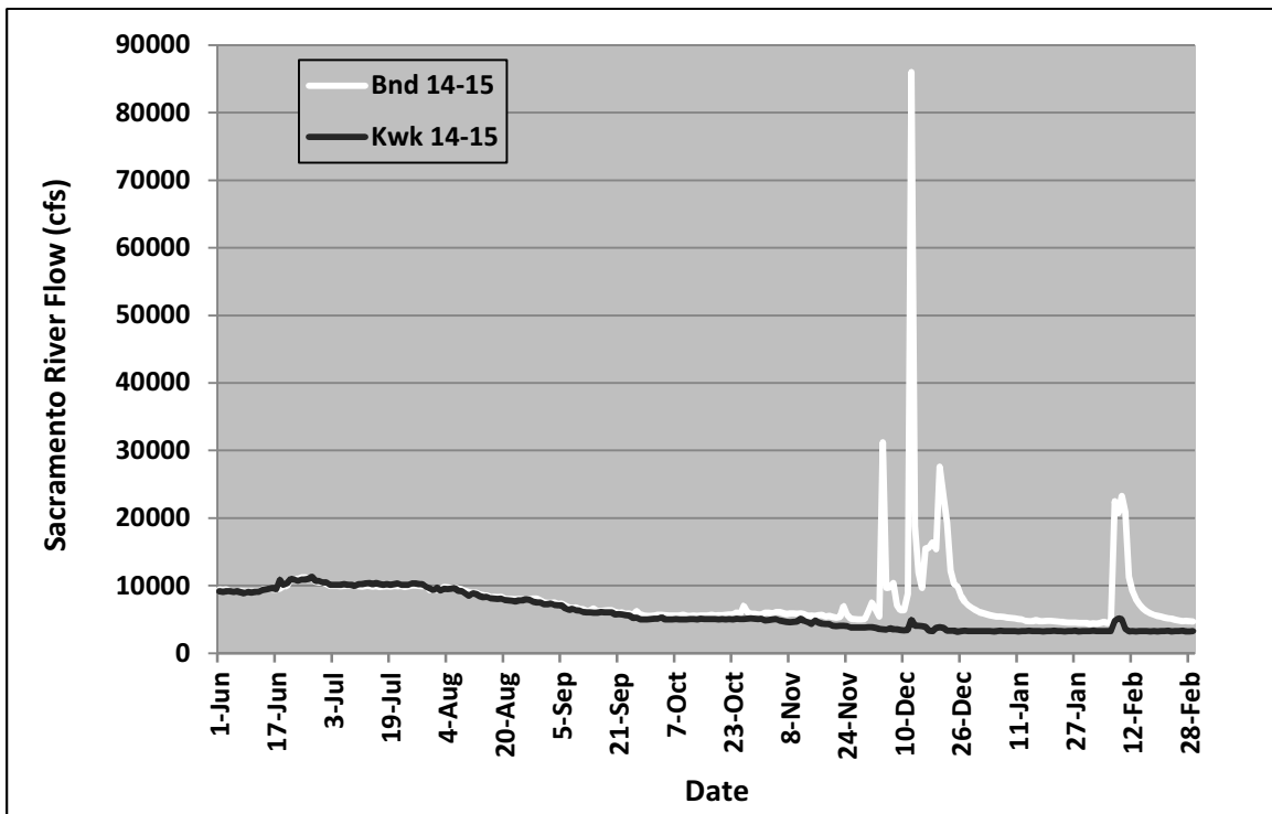
Figure 13. Graph of Sacramento River flow at KWK (below Keswick Dam) and at Bend Bridge (located 44 miles downstream of KWK) during study year 2014-2015.
