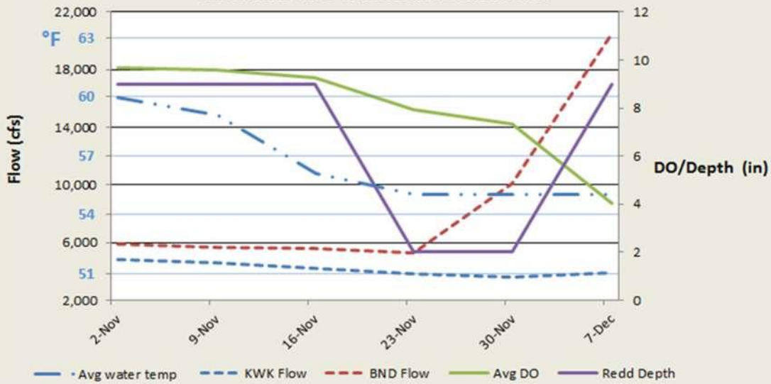
Average Weekly DO, Temperature, Flows and Water Depth by Date Sacramento River Mile 269: inside Redd #1337
