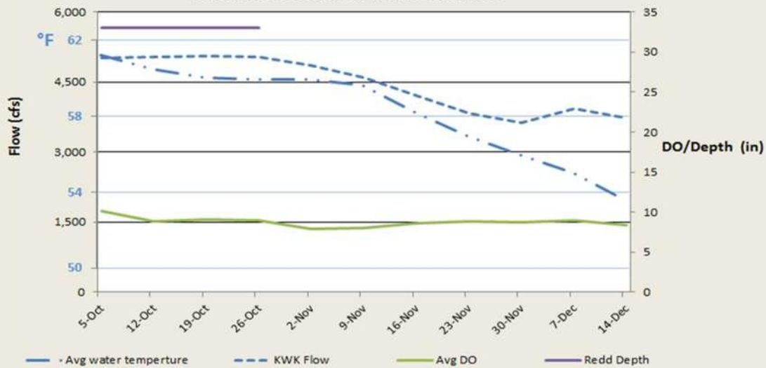
Average Weekly DO, Temperature, Flows and Water Depth by Date Sacramento River Mile 297: inside Redd #1071
