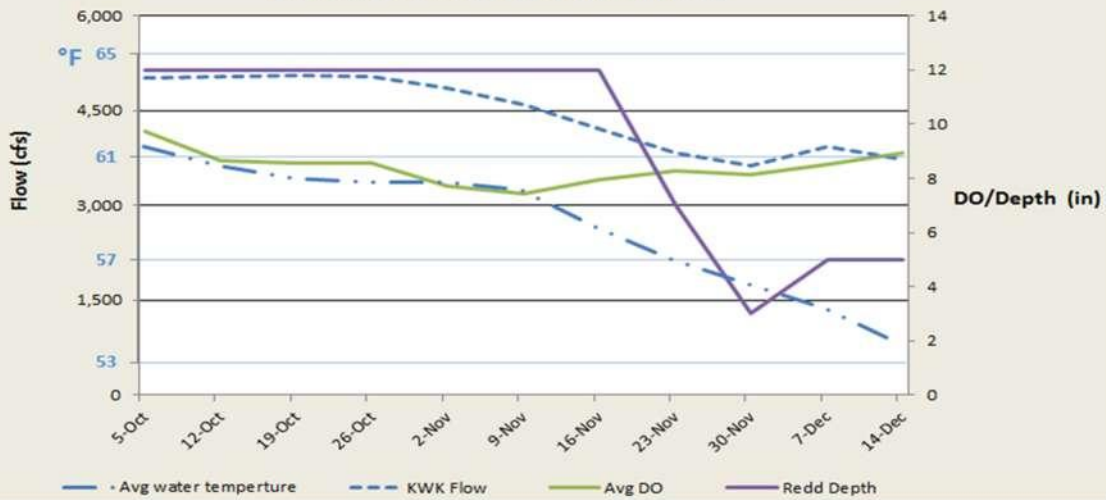
Average Weekly DO, Temperature, Flows and Water Depth by Date Sacramento River Mile 296: inside Redd #1070
