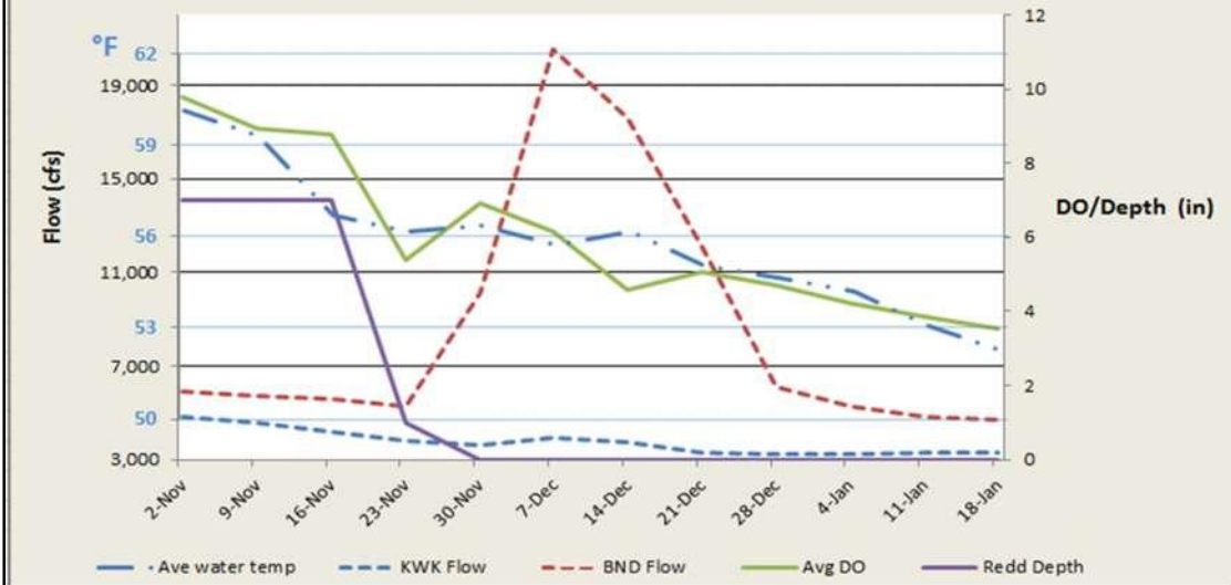
Average Weekly DO, Temperature, Flows and Water Depth by Date Sacramento River Mile 263: inside Redd #1327
