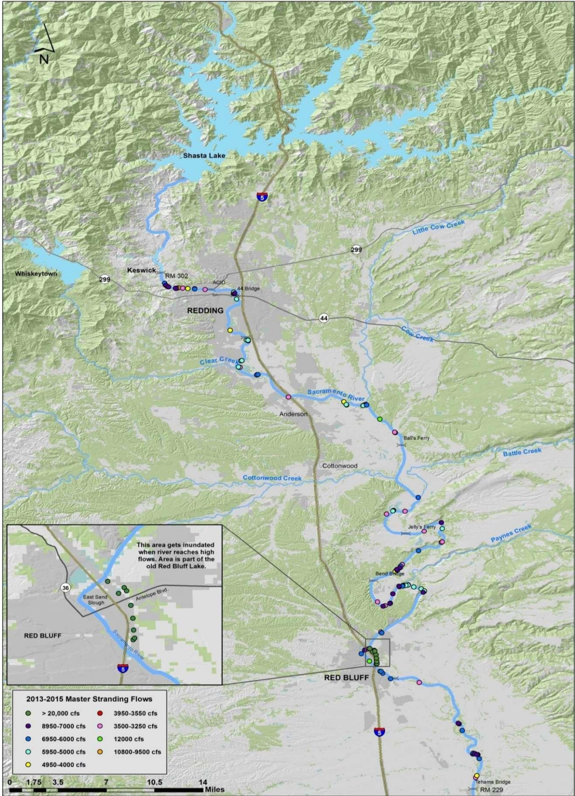
Appendix D Figure D5. Map of all 2013-2015 isolated stranding site locations. Sites are color coded based on the corresponding stranding flow range.
