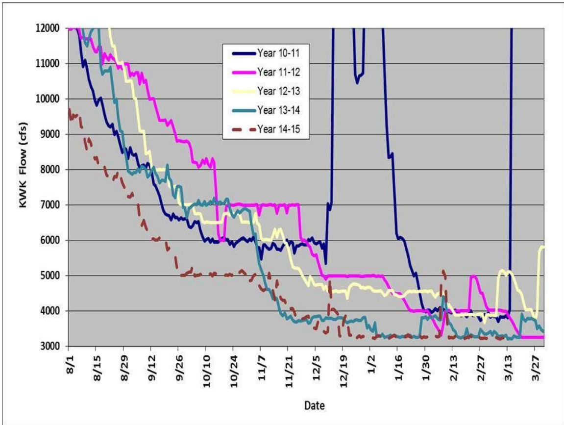
Figure 14. Graph of five years of Keswick Dam flows to the Sacramento River for the dates of interest to the dewatered redds and juvenile stranding study. Years 2013-2015 use the KWK flow gauge, other years use KES.
