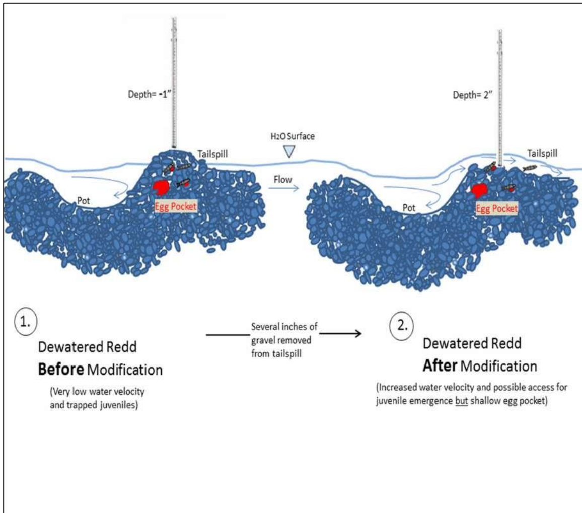
Figure 9. Diagram of the redd modification process. Redd water depths and velocities are measured before and after substrate is removed from the tailspill. Redd modification increases the water velocity over a redd and likely allows juvenile salmon to emerge successfully but decreases the egg pocket depth. Note: redd dimensions are not to scale. Egg pocket depths vary within each redd.
