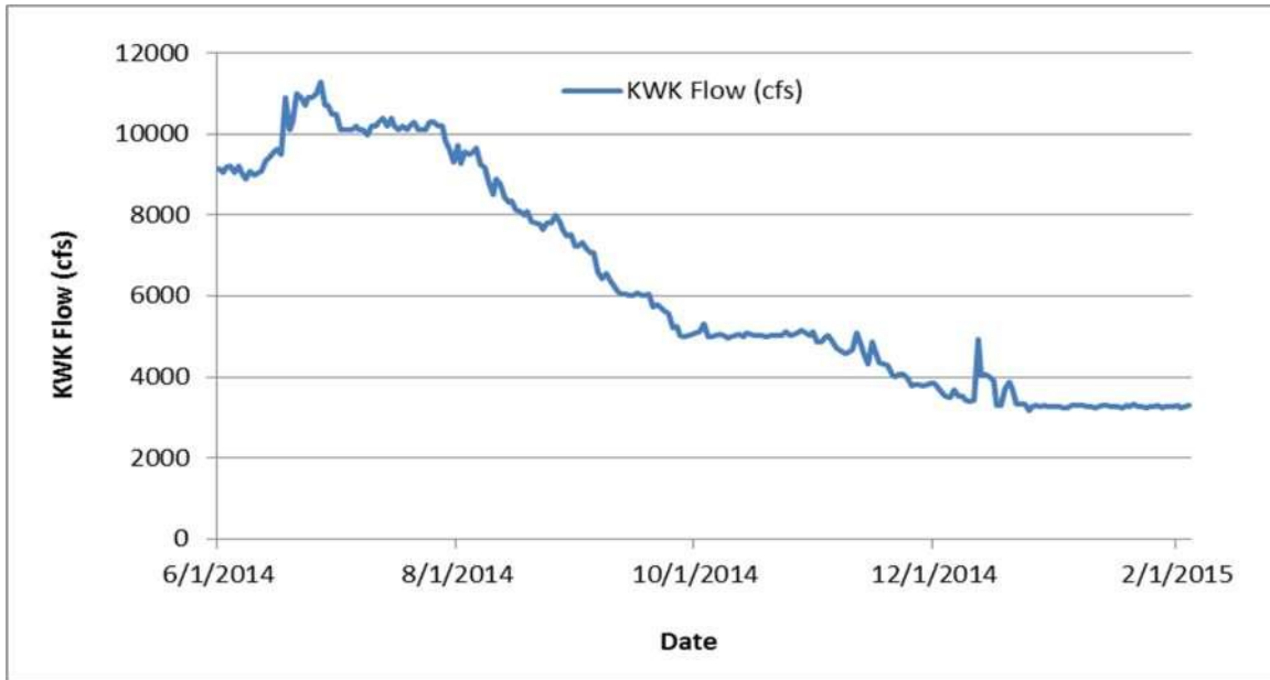
Figure 2. Flow releases from Keswick Dam on Sacramento River during selected periods in 2014 and 2015, from internet KWK-USGS gauge (CDEC, 2015).
