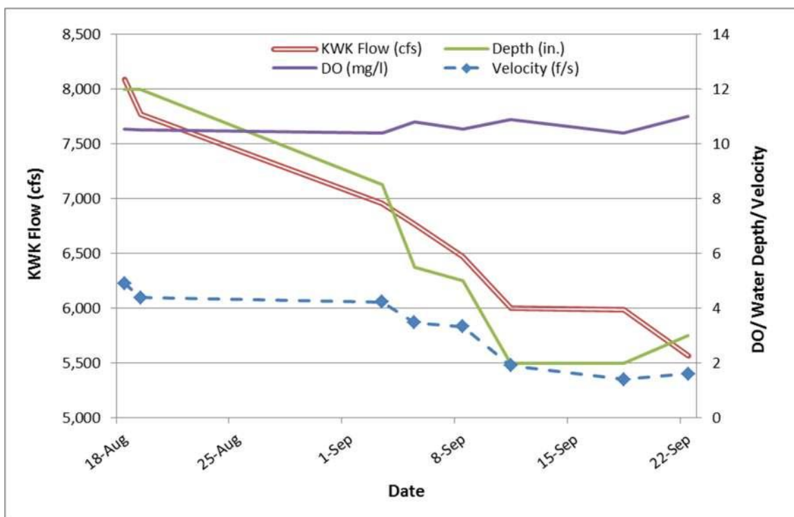
Figure 6. An example of water quality measurements collected during 2014 on a winter-run redd and compared to flow. Note: this redd was modified on September 18. Data collected on September 22 displays an increase in depth.
