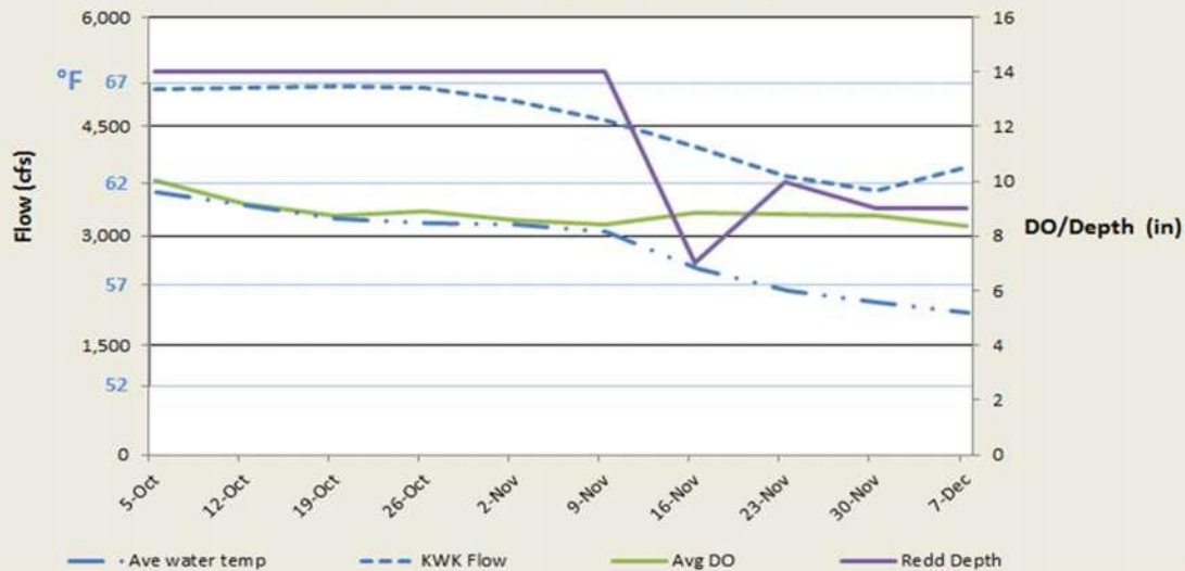
Average Weekly DO, Temperature, Flows and Redd Depth of Logger:
