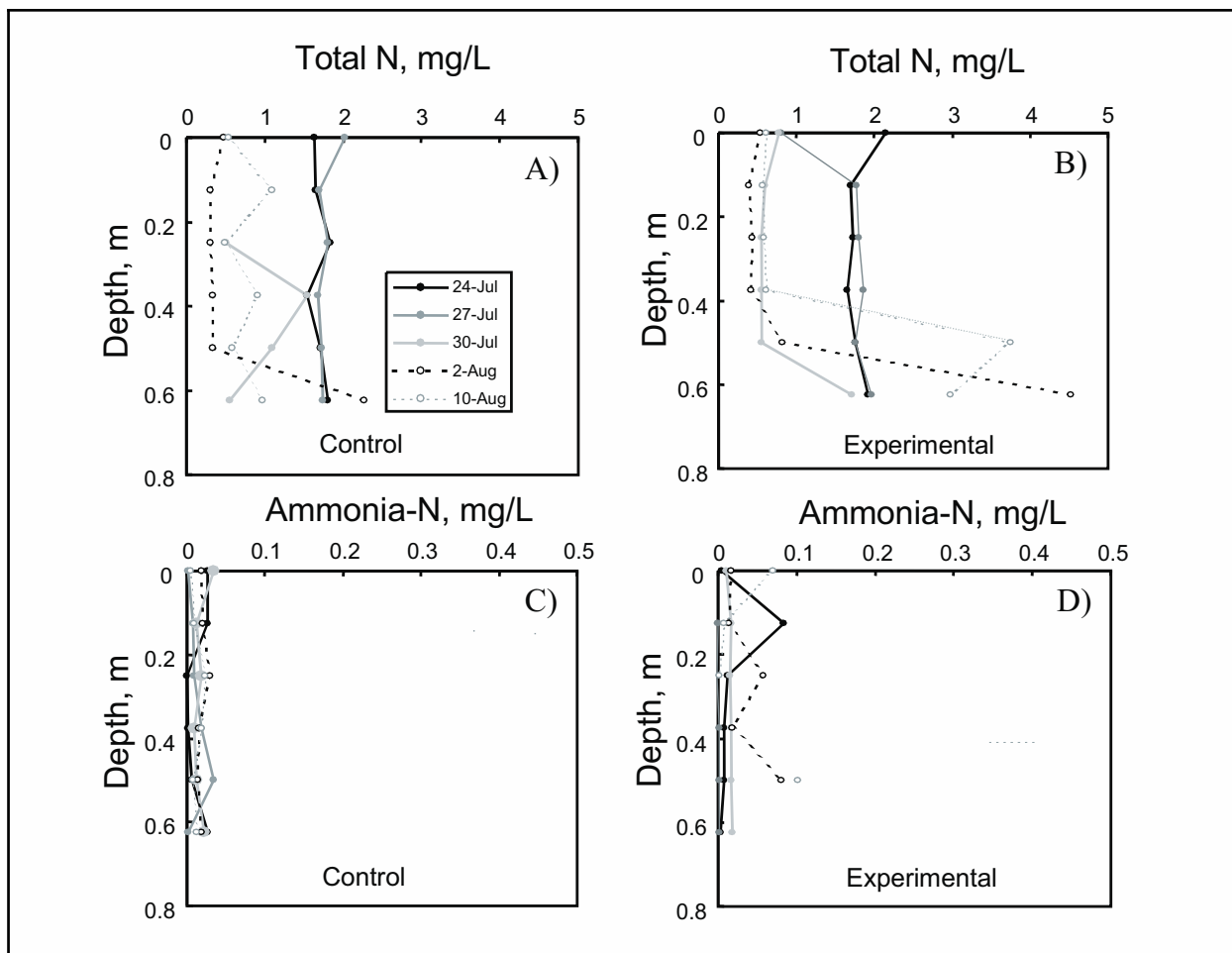
Figure 3. Variations in total nitrogen (TN) and ammonium-N (NH 3 -N) in the water column at the control and experimental stations. Mechanical shredding occurred at the experimental site on 26 July 1999
