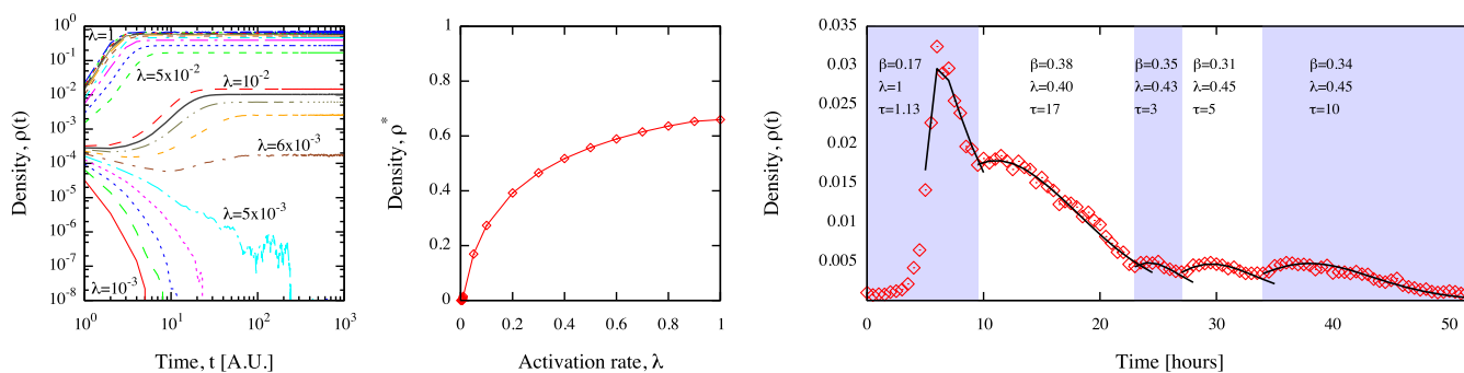
Figure 8 | First panel: Evolution of the density of active users versus time obtained from simulations of spreading dynamics. The de-activation rate is \beta = 1 and the different curves correspond to different values of the activation rate \lambda . Each curve corresponds to the ensemble average of 200 random independent realizations. Second panel: Average value of the density of active users in the stationary state, as a function of \lambda . Third panel: Observed evolution of the density of active users versus time (points) in Period IV, i.e., during and after the main event, from 03:00 AM, 4 th July. Curves indicate the predictions obtained from the model defined by Eq. 8 coupled to Eq. 9, where the values of the corresponding parameters are reported in the figure for different sub-periods. The reported \lambda refers to the initial value of the activation rate.
