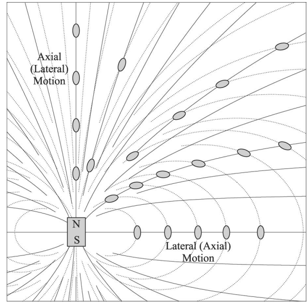
Fig. 7. Translation paths of a body as it is attracted to a magnetic dipole. Magnetic field lines are shown (· · ·). Force lines are also shown (—), assuming that the long dimension of the body is aligned with the field. The body will typically rotate as it is attracted toward the dipole, but pure axial and lateral translations of the body are possible, as shown for prolate (oblate) bodies.
