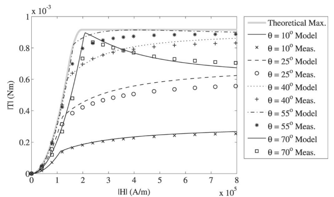
Fig. 4. Modeled and measured torque magnitude versus applied field strength for various applied field angles.
