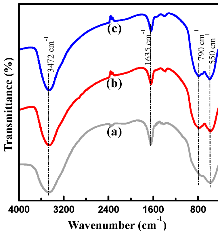
Figure S2. The FTIR spectra recorded for ALVIR, RAWOS and RAWS catalysts (a–c).
