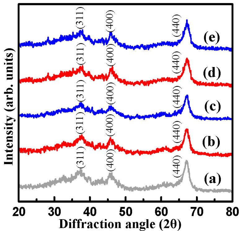
Figure S1. The XRD spectra of the catalysts: The as prepared ALVIR (a); RAWOS (b); and RAWS (c). The RAWOS and RAWS catalysts heat-treated at 650° C are given in (d) and (e), respectively.
