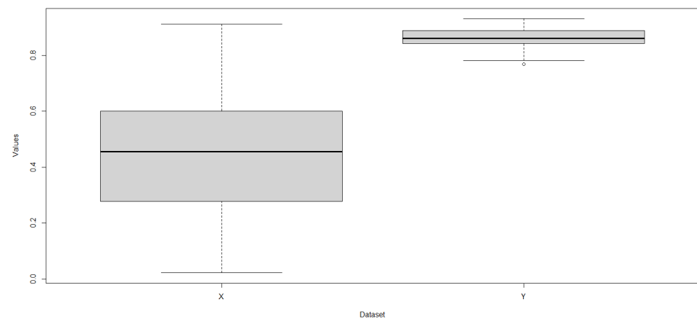
Figure 4. Boxplots of X (left) and Y (right).
