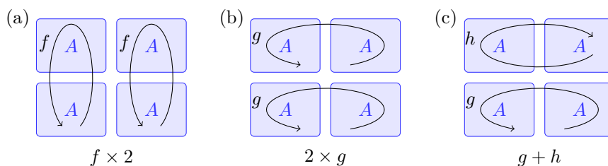
Figure 1: Visualizing permutations of 2 \times A \times 2
