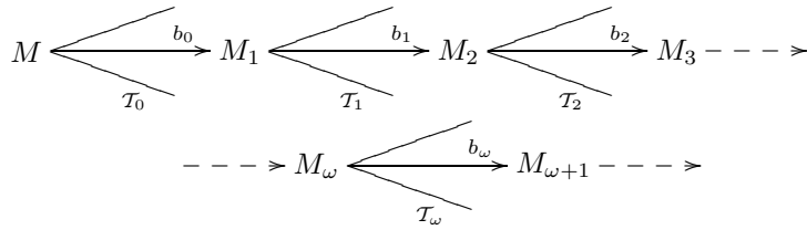
DIAGRAM 6. An iteration game.
