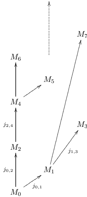
DIAGRAM 5. A sample iteration tree, with the tree order 0 T 1, 0 T 2, 1 T 3, 1 T 7, \dots
