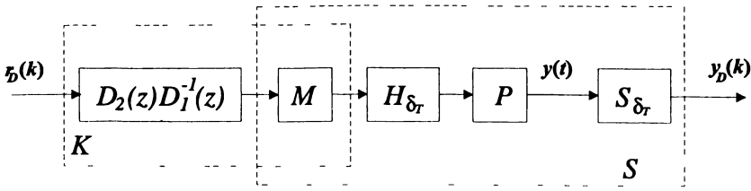
Fig. 4. Factorisation of compensator K .
