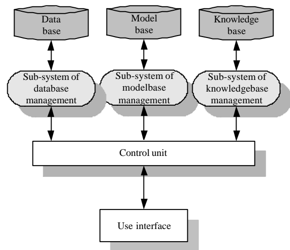
Fig. 1 Basic structure of SDSS
