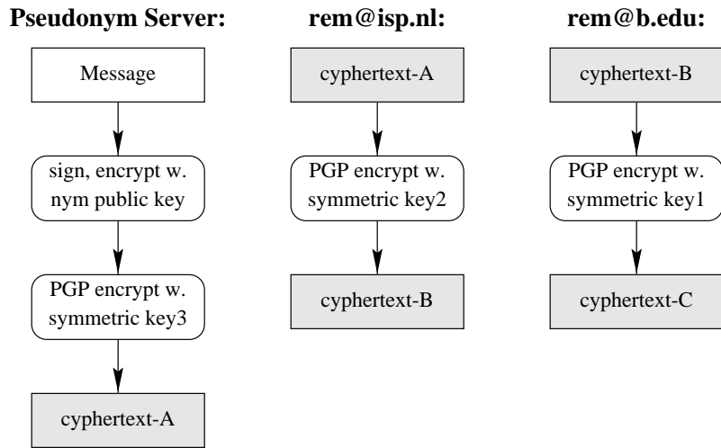
b. Encryptions performed on messages at each remailer
