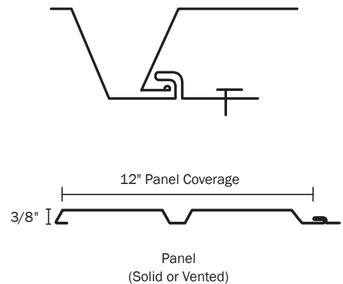
E-375 3/8" Soffit Panel
