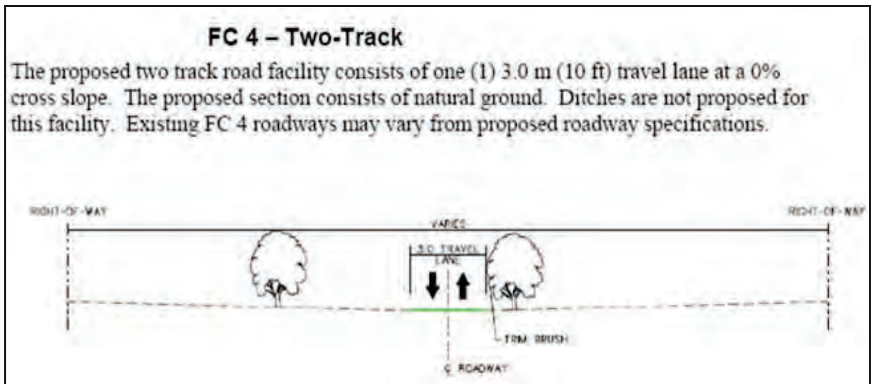
Figure B-8. FC-4 Two-Track Road (Diagram)
