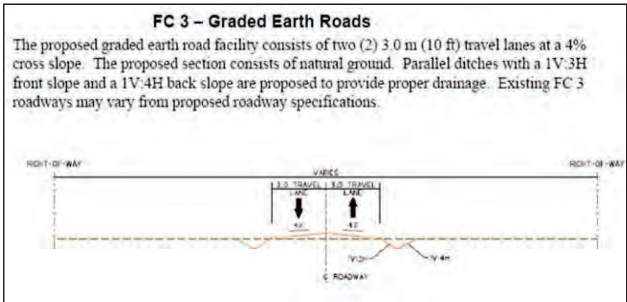
Figure B-6. FC-3 Graded Road (Diagram)
