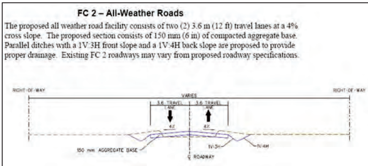
Figure B-4. FC-2 All-Weather Road (Diagram)
