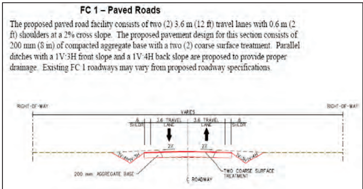
Figure B-2. FC-1 Paved Road (Diagram)
