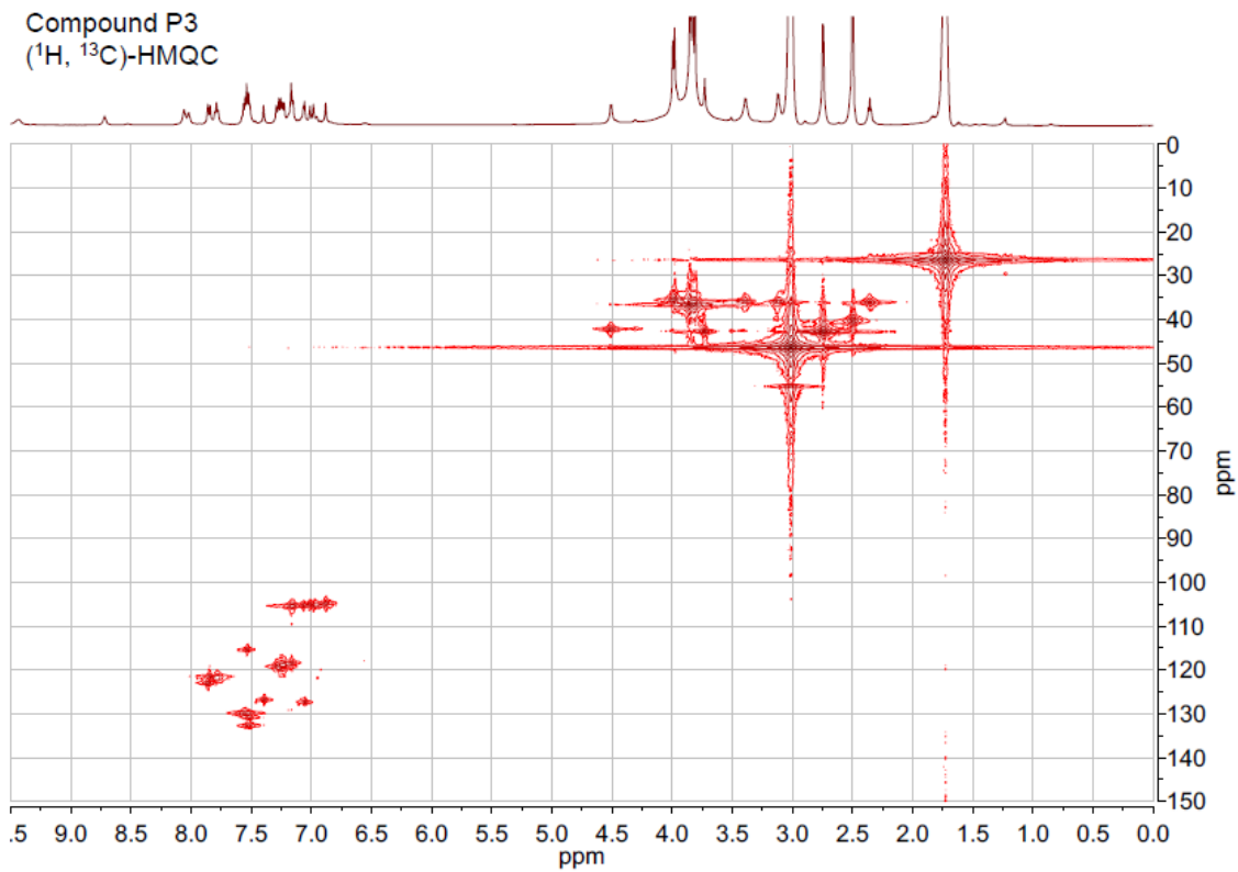
Compound P3 ( 1 H, 13 C)-HMBC
