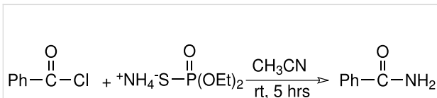
Scheme 5: Reaction of ammonium O,O' -diethyl thiophosphate with benzoyl chloride
