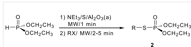
Scheme 7: Synthesis of phosphorothioates using triethylammonium O,O' -diethyl thiophosphate using microwave irradiation.
