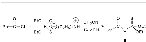
Scheme 6: Reaction of triethylammonium O,O' -diethyl thiophosphate with benzoyl chloride
