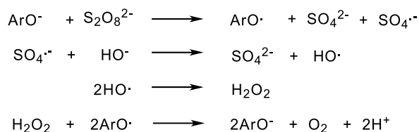
Scheme 7: A Catalytic Cycle for Peroxydisulfate Consumption.
