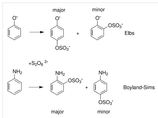
Scheme 1: The Elbs and Boyland-Sims Oxidations.
