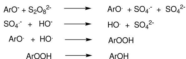
Scheme 8: A Non-catalytic cycle for Peroxydisulfate Consumption.
