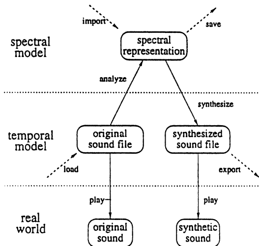
Figure 1: InSpect Architecture
