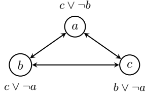
Figure 5: The ADF of Example 4
