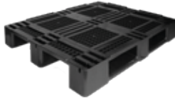
APD3-PE G Premium Open Deck Plastic Pallet D: 1200 x 1000 x 150mm W: 14kg Load Capacity: 5000kg
