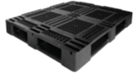
APD3-5 PE G Premium Open Deck Plastic Pallet D: 1200 x 1000 x 150mm W: 15kg Load Capacity: 5000kg
