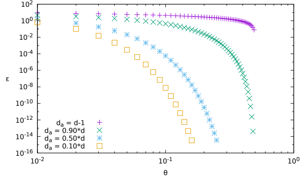
Fig. 3. Sparse-PIR: \epsilon versus \theta for d = 100
