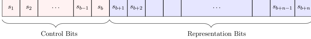
Figure 2: Illustration of state for majority MDPs.
