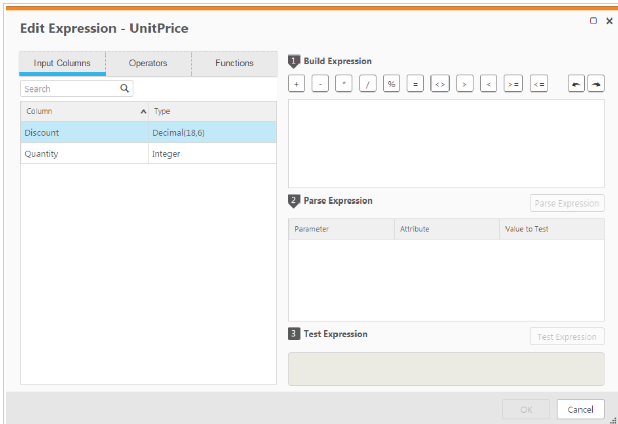
Figure 6.1 | Expression Builder
