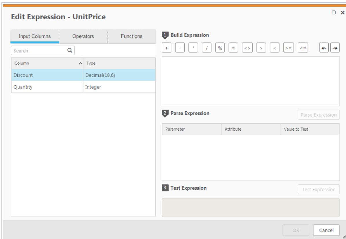
Figure 6.1 | Expression Builder
