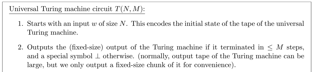
Figure 2: Universal Turing machine circuit
