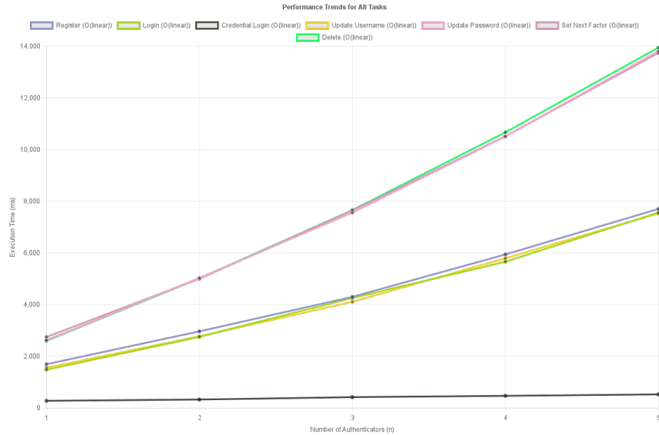
Fig. 1. Performance trend of COCO protocol tasks. Execution times are plotted against the number of authenticators.
