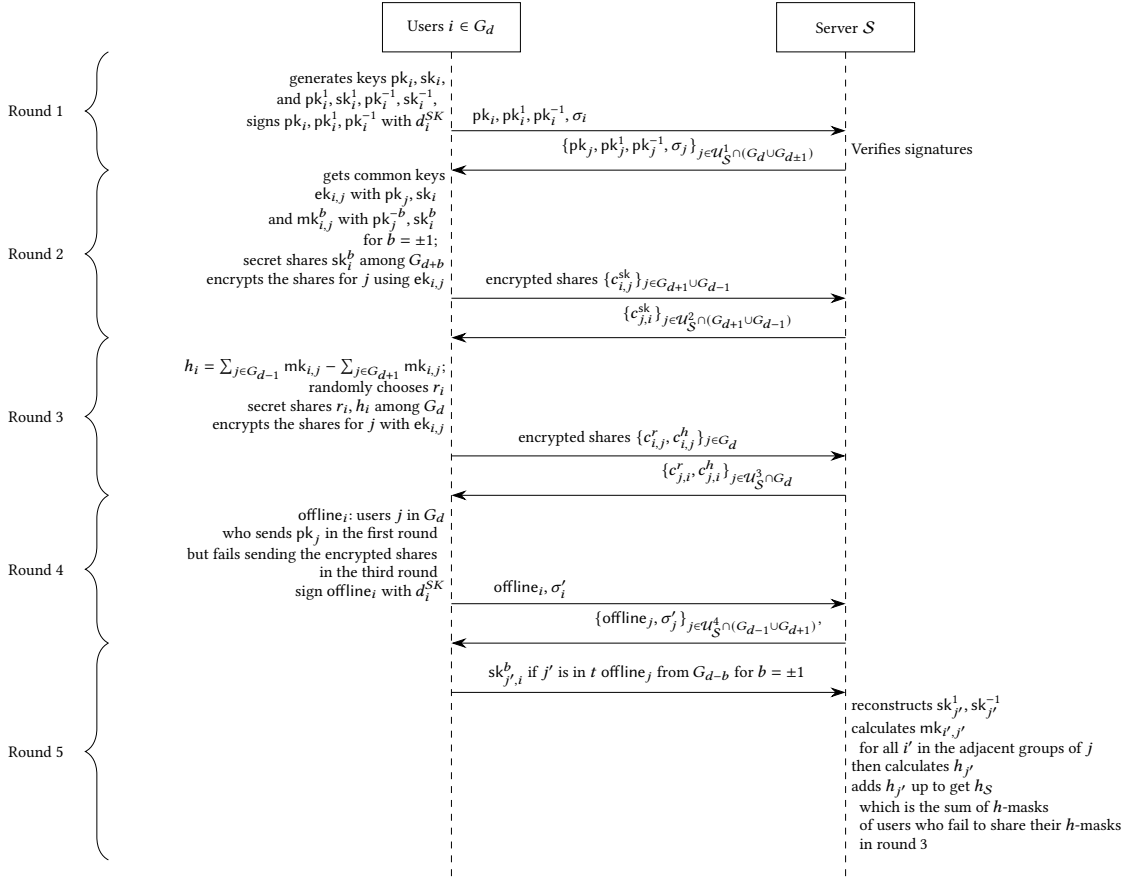
Figure 7: An overview of the Setup phase of MicroSecAgg gDL
