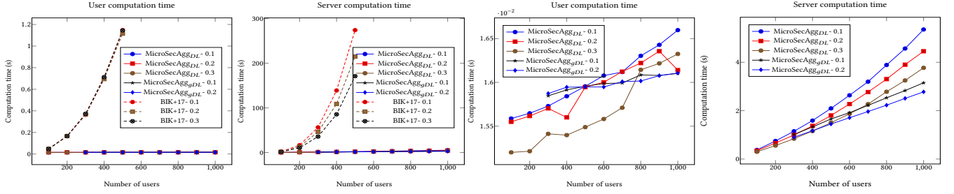
Figure 10: The left two graphs show wall-clock computation time of one iteration of the aggregation phase as the number of users increases. Different lines show the running time with different offline rates which is indicated in the legend, e.g., 0.1 means 10% of users are offline. The length of the output is fixed to 16 bits. The right two graphs are zoom-in with only \text{MicroSecAgg}_{DL} and \text{MicroSecAgg}_{gDL} included.
